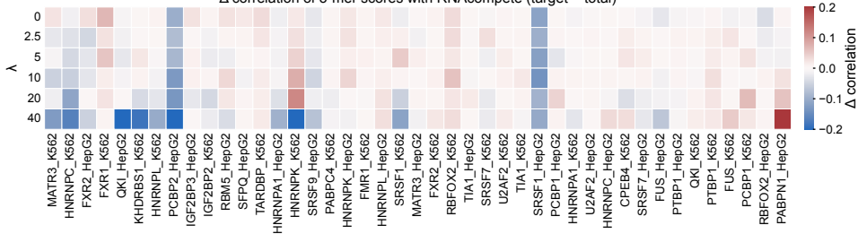
Δ correlation of 5-mer scores with RNAcompete (target – total)
