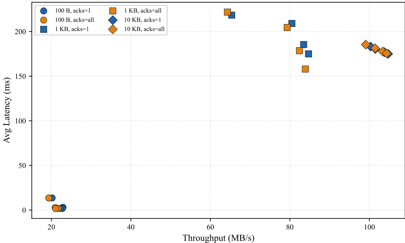
Throughput vs. Latency Tradeoff (1M msg/s target)
