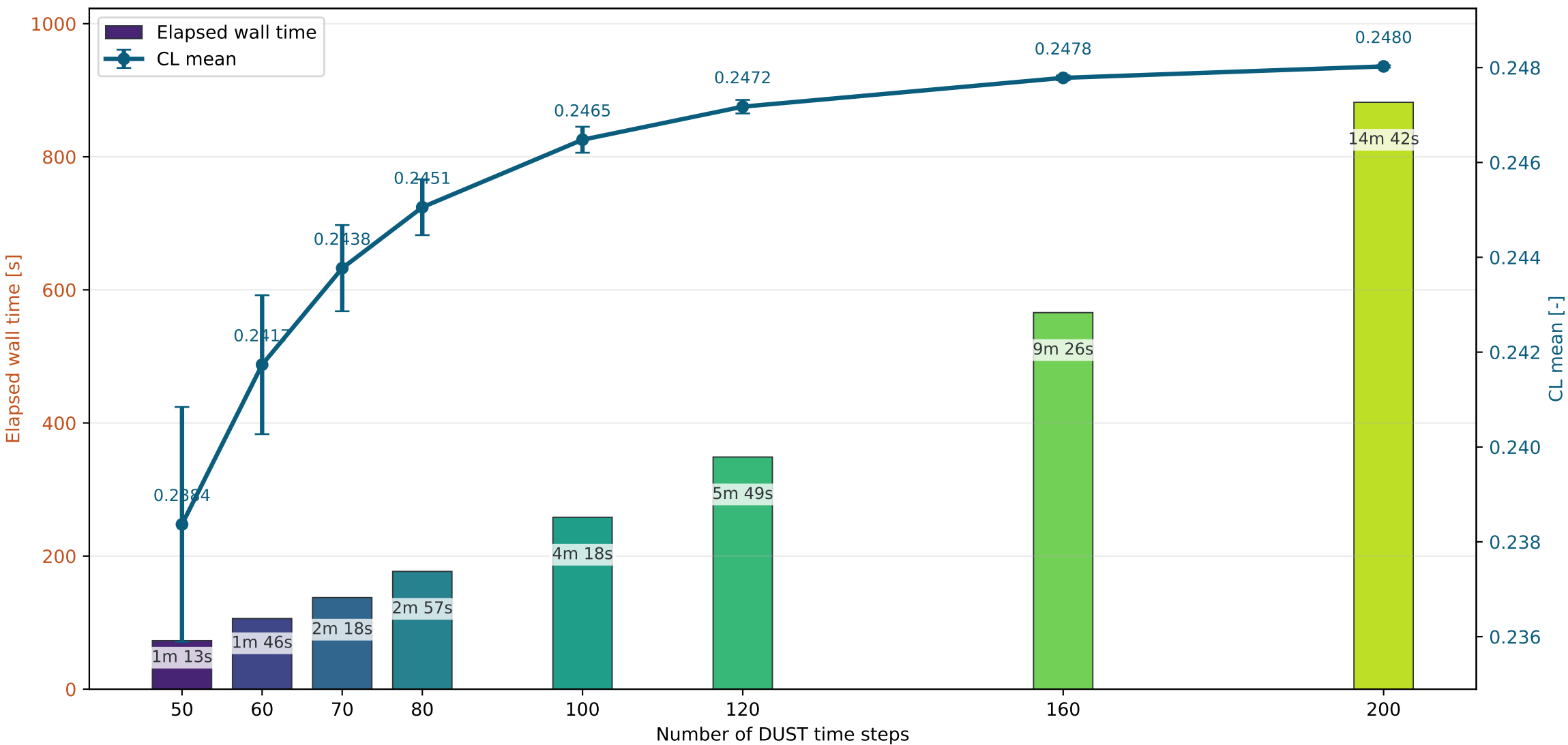
CTA DUST panel convergence: runtime vs CL mean
