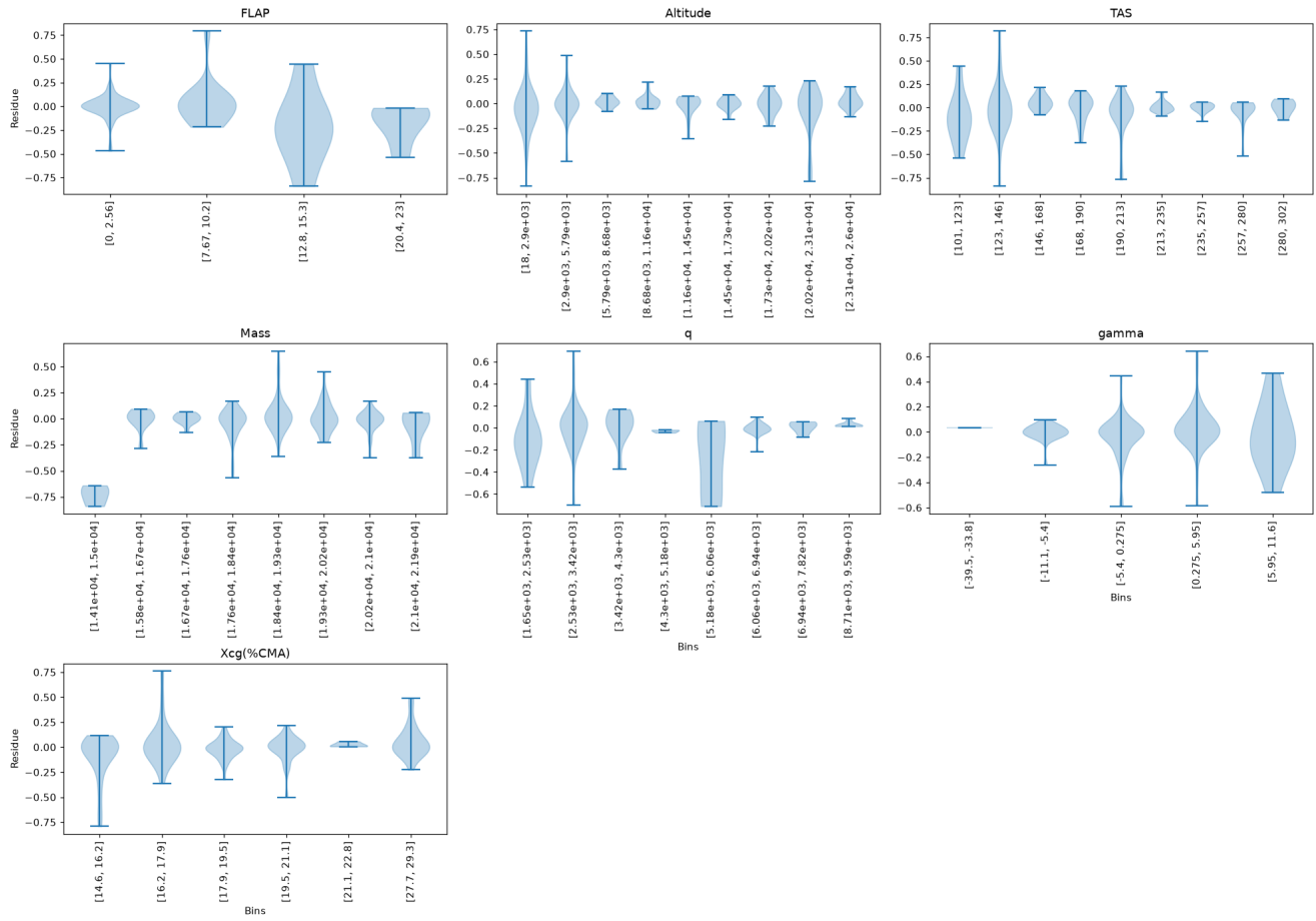
Turn Violin plot [Bins vs Residue] inside \mu \pm 3\sigma
