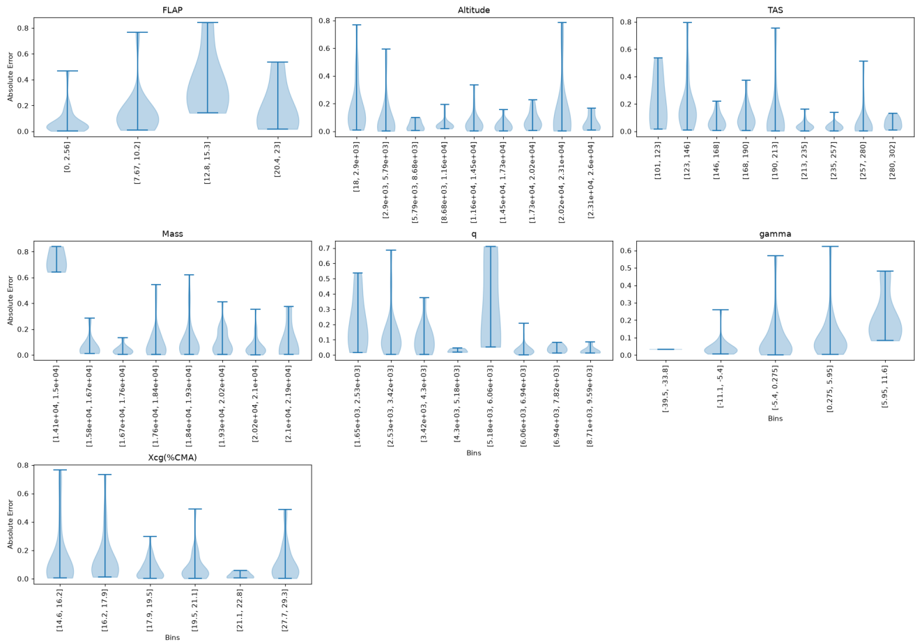
Turn Violin plot [Bins vs Absolute Error] inside \mu \pm 3\sigma
