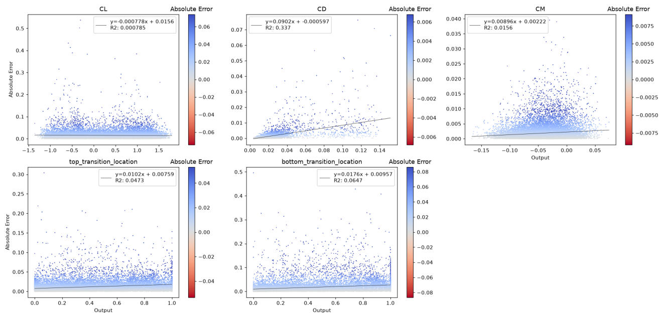
Scatter plot [Output vs Absolute Error] (color trimmed to \mu \pm 3\sigma )
