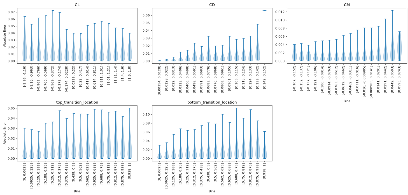
Violin plot [Bins vs Absolute Error] inside \mu \pm 2\sigma
