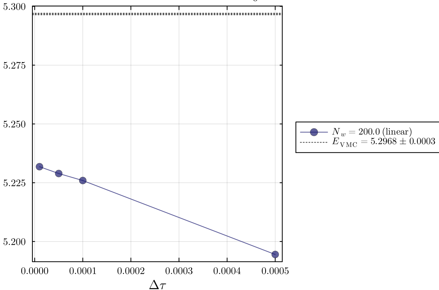
DMC Energy vs \Delta\tau , N = 30 , nr_0^2 = 16
