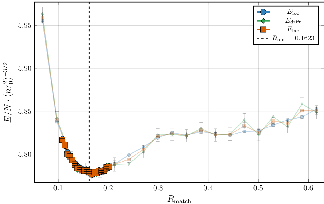
R_{\text{match}} Optimization, nr_0^2 = 16 , N = 30
