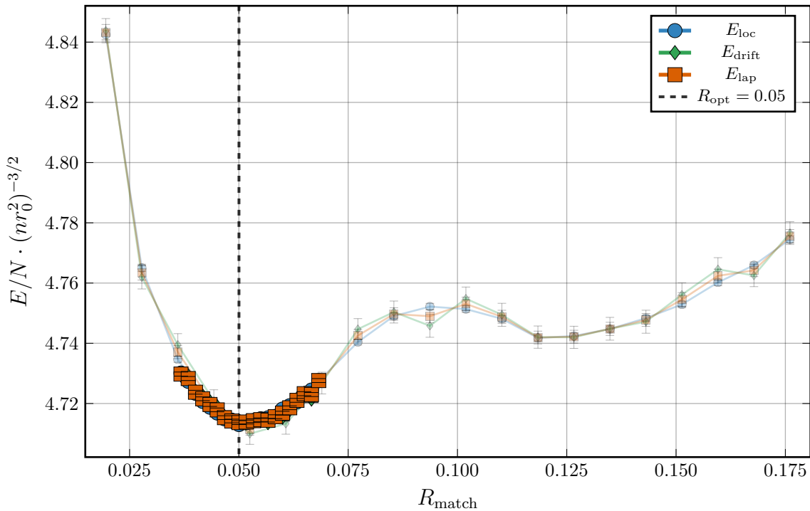
R_{\text{match}} Optimization, nr_0^2 = 196 , N = 30
