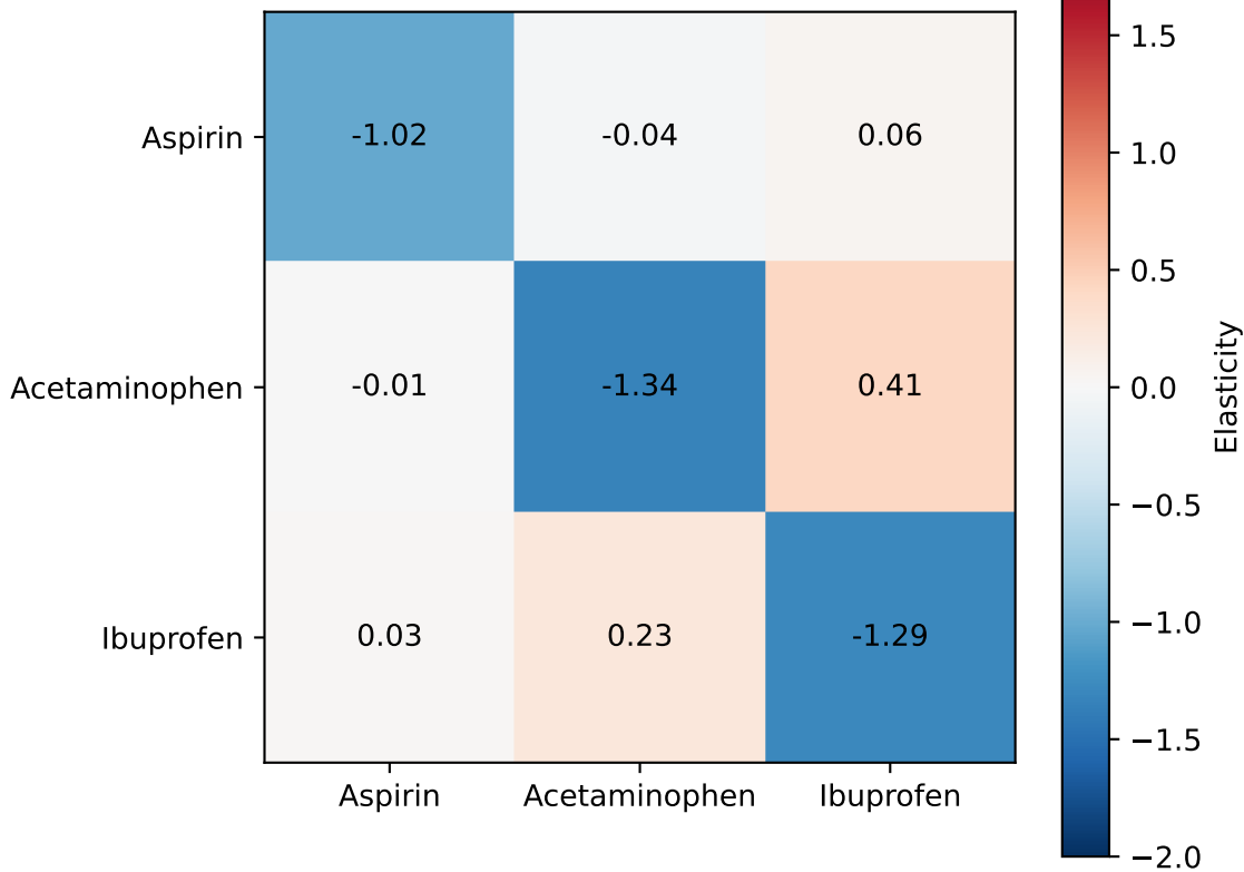
Cross-Price Elasticities — Neural Demand (habit, )
