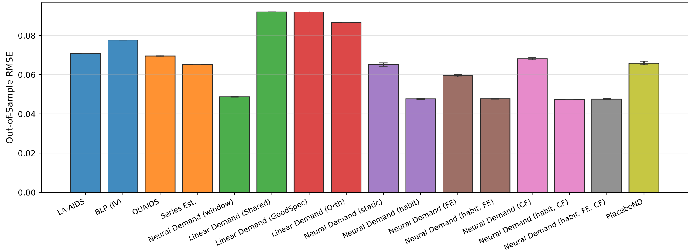
Out-of-Sample RMSE — Mean \pm 1 SD (5 runs) Dominick's Analgesics
