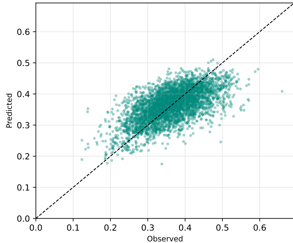
Ibuprofen RMSE=0.0524
