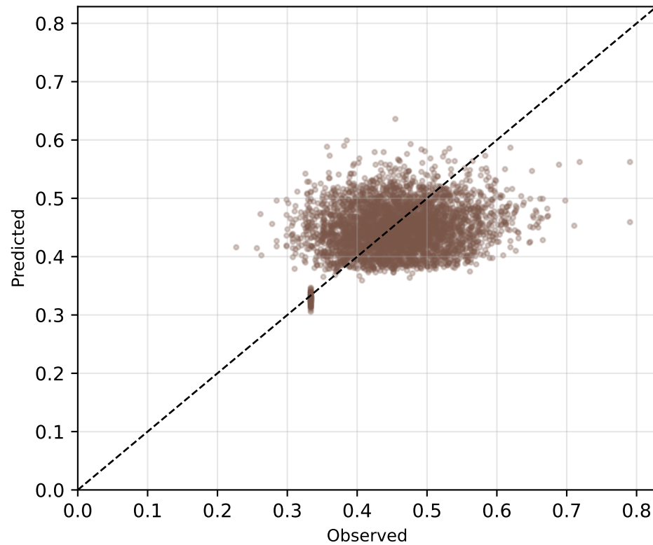
Acetaminophen RMSE=0.0697
