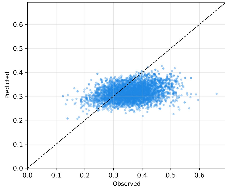
Ibuprofen RMSE=0.0790
