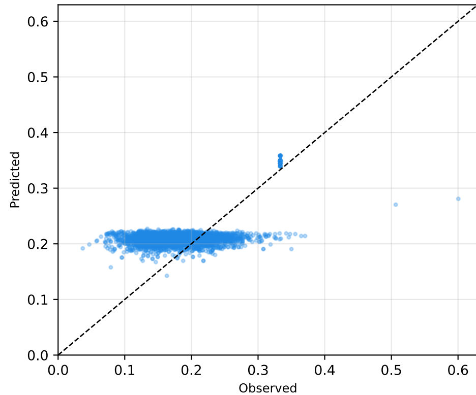
Aspirin RMSE=0.0507
