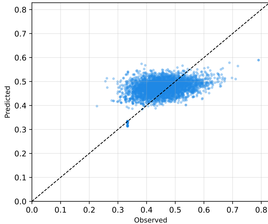
Acetaminophen RMSE=0.0630
