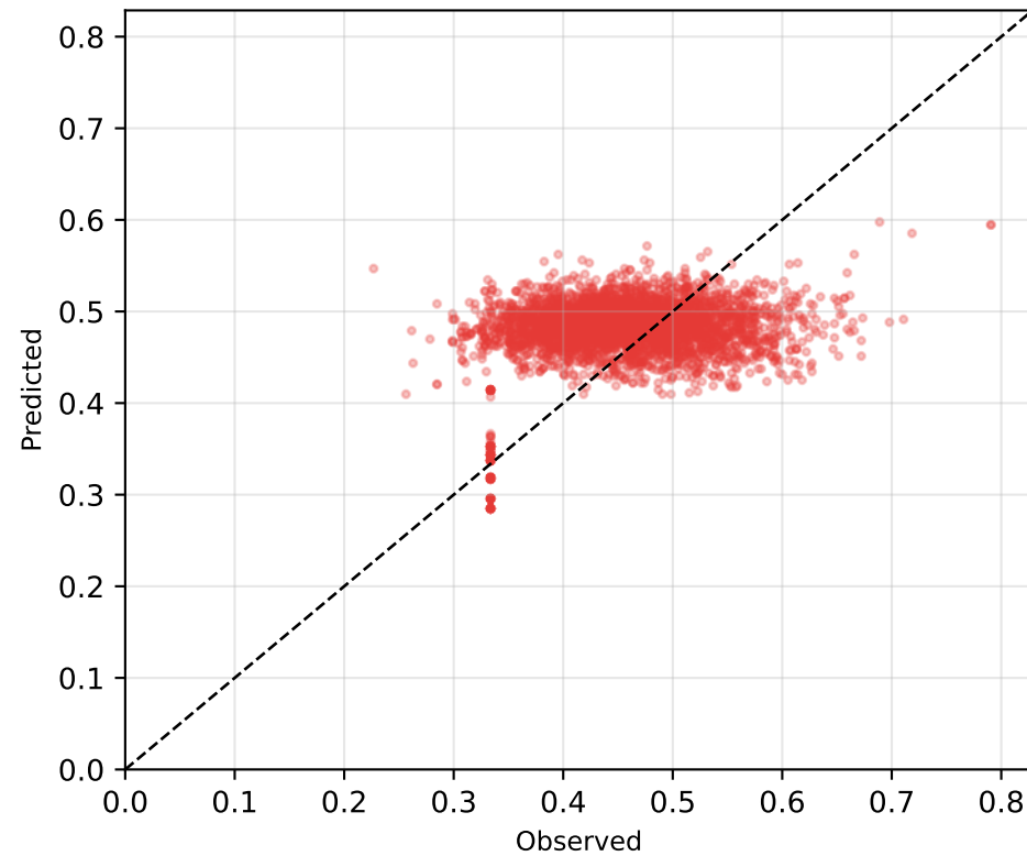
Acetaminophen RMSE=0.0712
