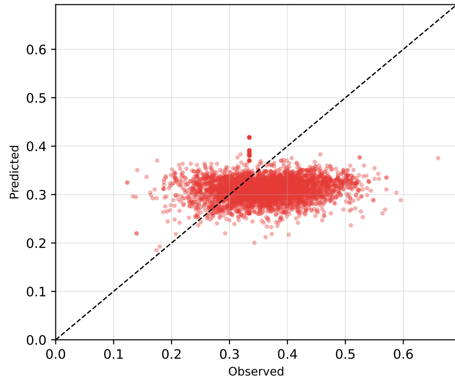
Ibuprofen RMSE=0.0858
