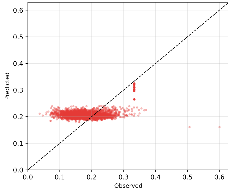
Aspirin RMSE=0.0506
