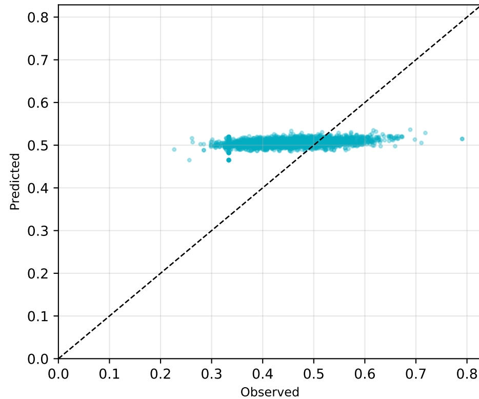
Acetaminophen RMSE=0.0867
