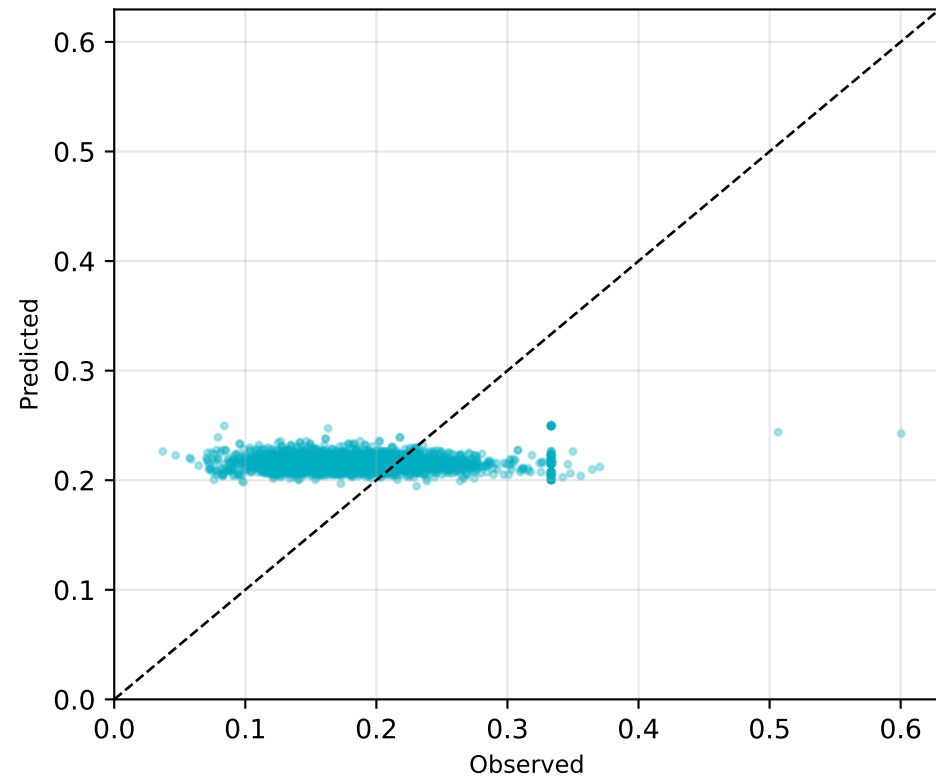
Aspirin RMSE=0.0622
