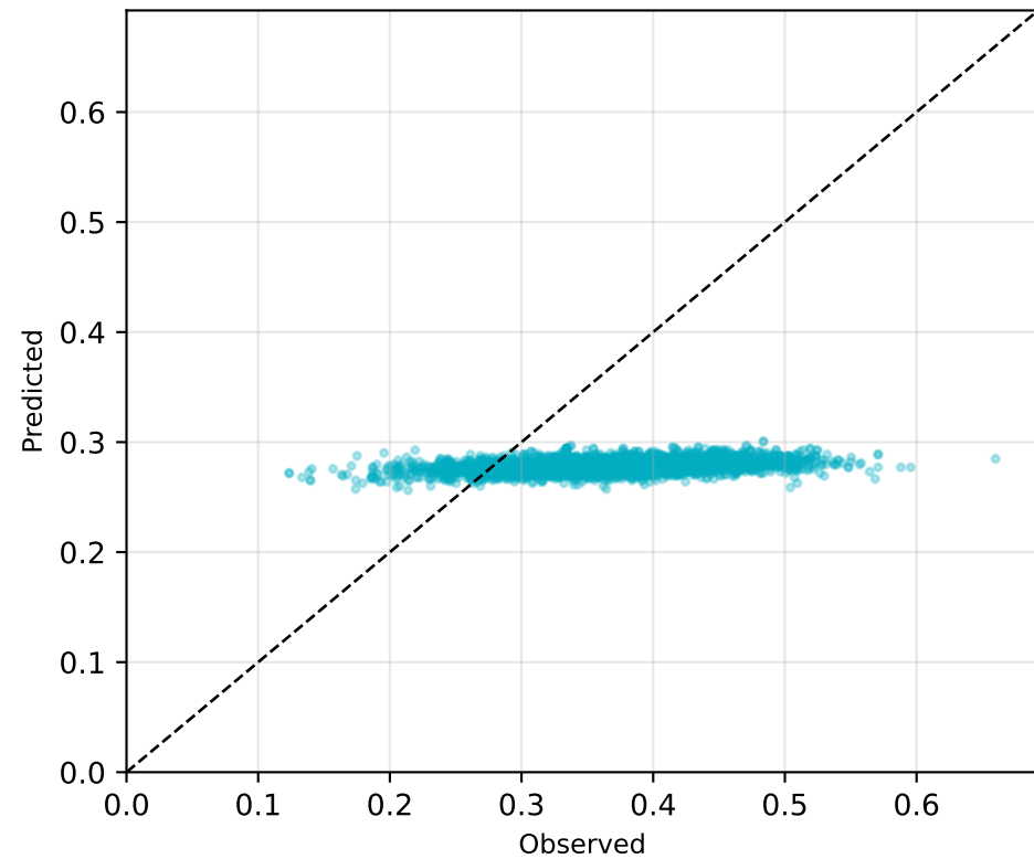
Ibuprofen RMSE=0.1055
