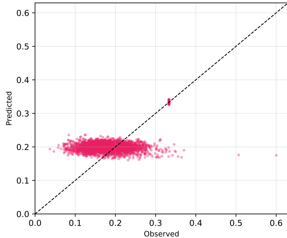
Aspirin RMSE=0.0477
