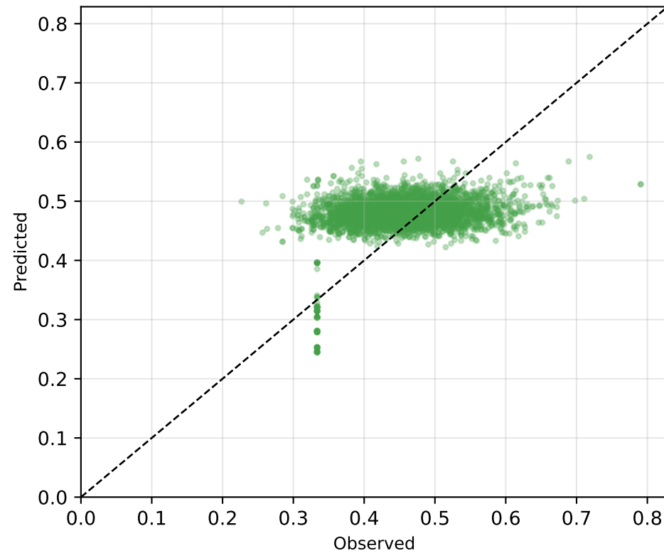
Acetaminophen RMSE=0.0686
