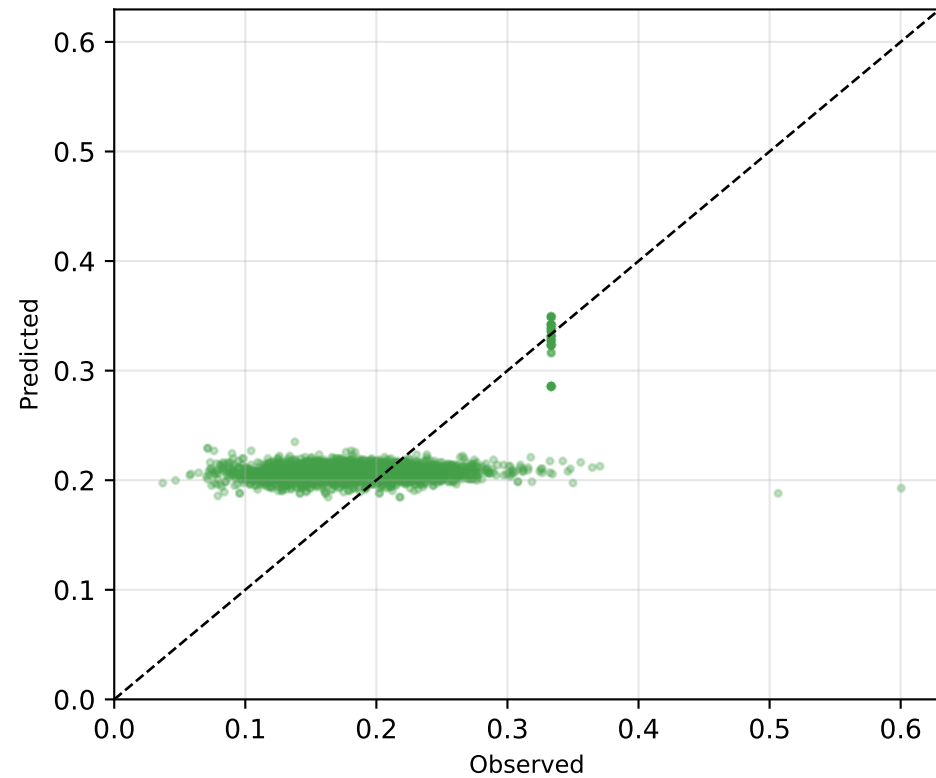
Aspirin RMSE=0.0504
