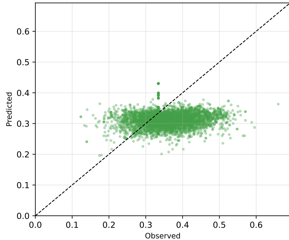
Ibuprofen RMSE=0.0853
