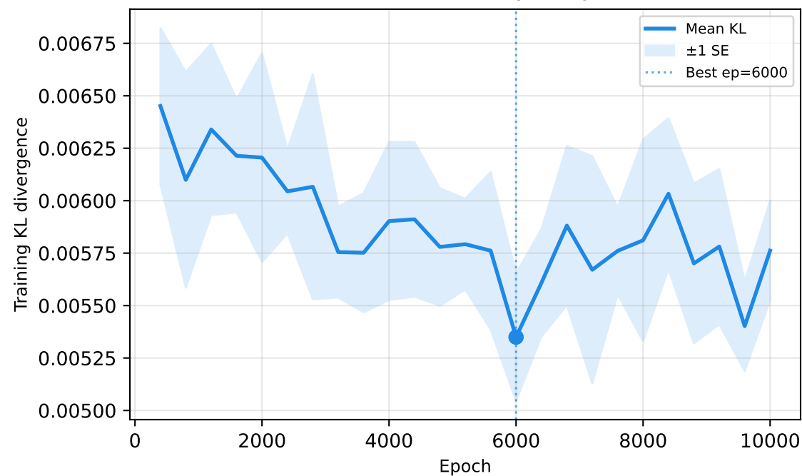
Neural Demand (CF)
