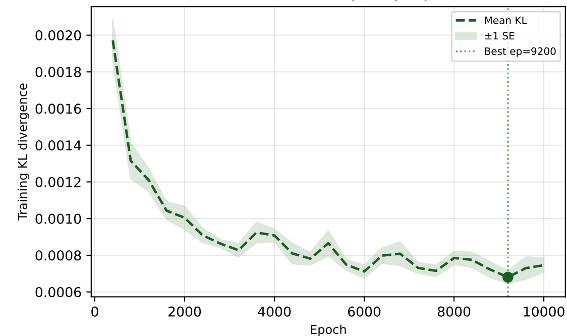
Neural Demand (habit, CF)
