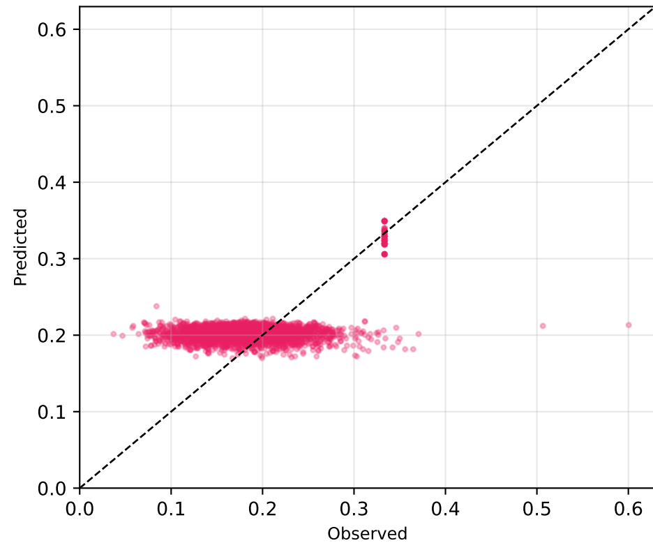
Aspirin RMSE=0.0483
