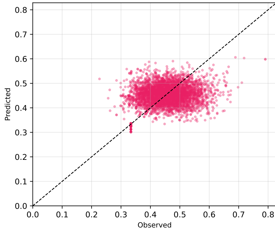
Acetaminophen RMSE=0.0714
