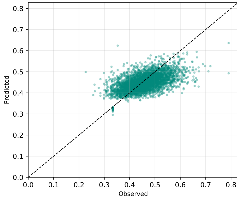
Acetaminophen RMSE=0.0534
