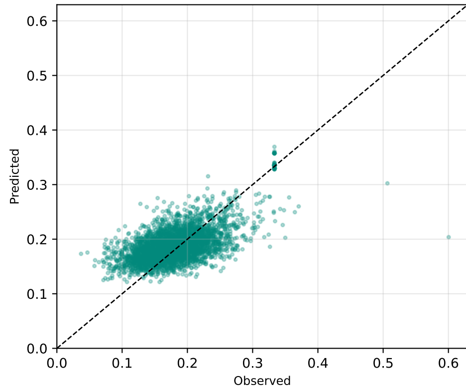
Aspirin RMSE=0.0365
