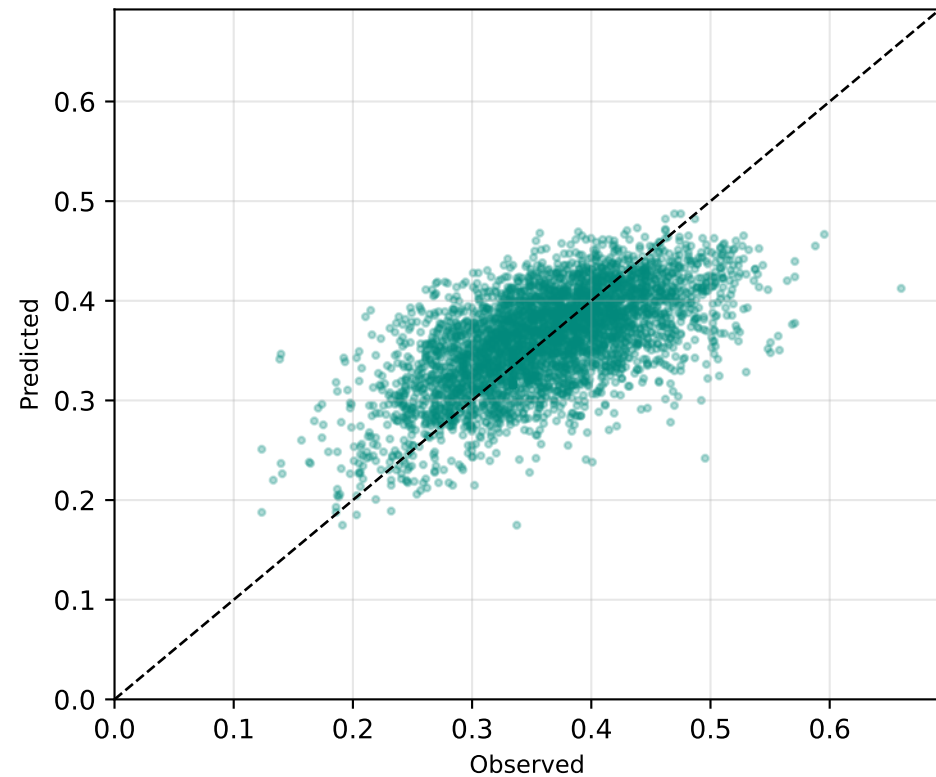
Ibuprofen RMSE=0.0522
