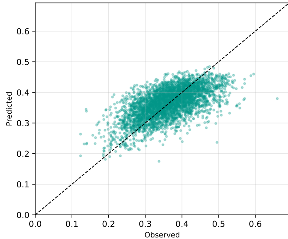
Ibuprofen RMSE=0.0523
