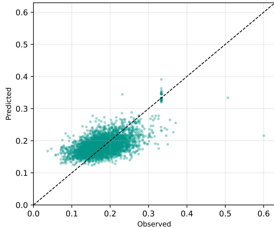
Aspirin RMSE=0.0365
