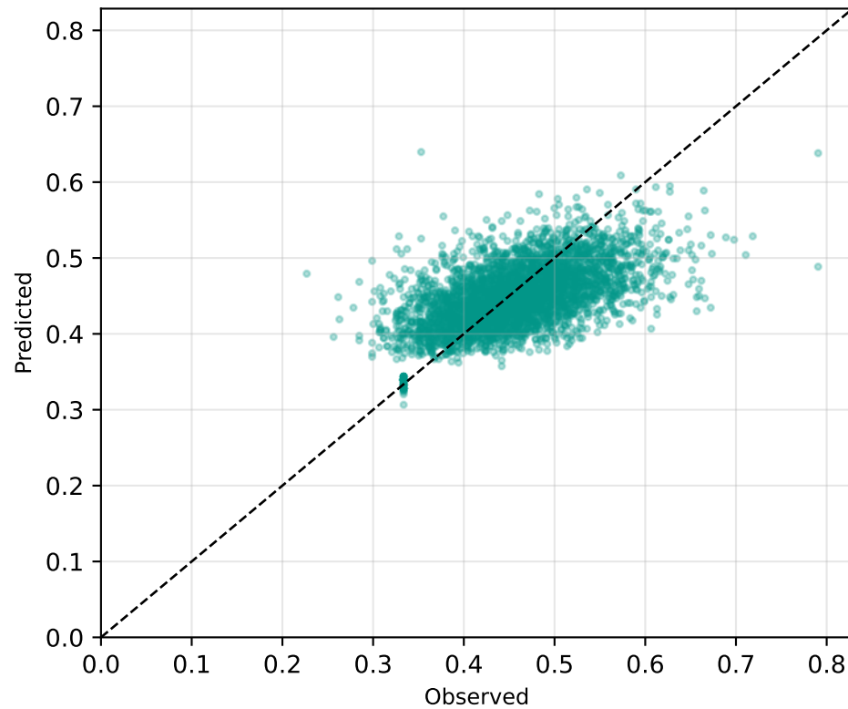
Acetaminophen RMSE=0.0536
