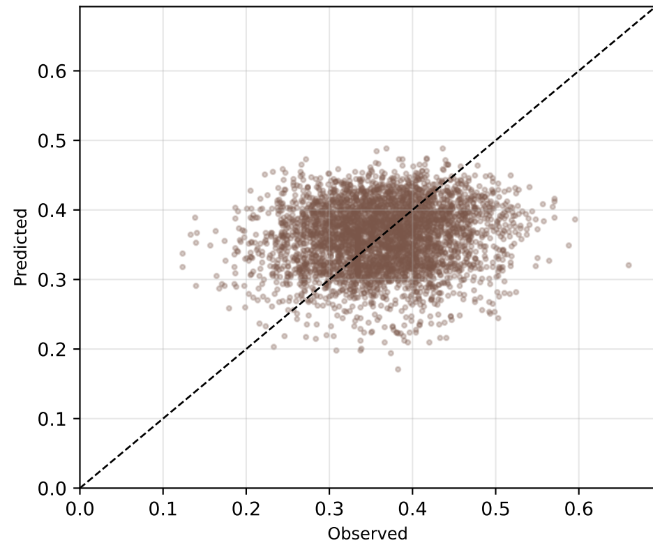
Ibuprofen RMSE=0.0761
