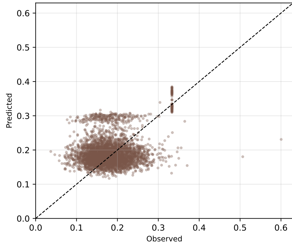
Aspirin RMSE=0.0546
