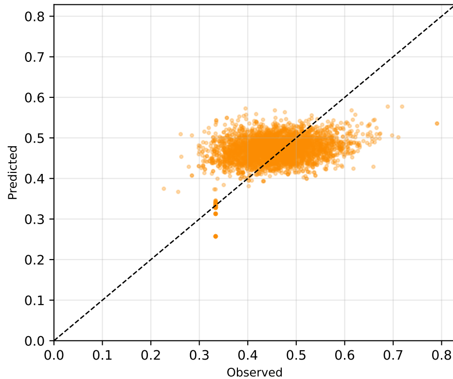
Acetaminophen RMSE=0.0644
