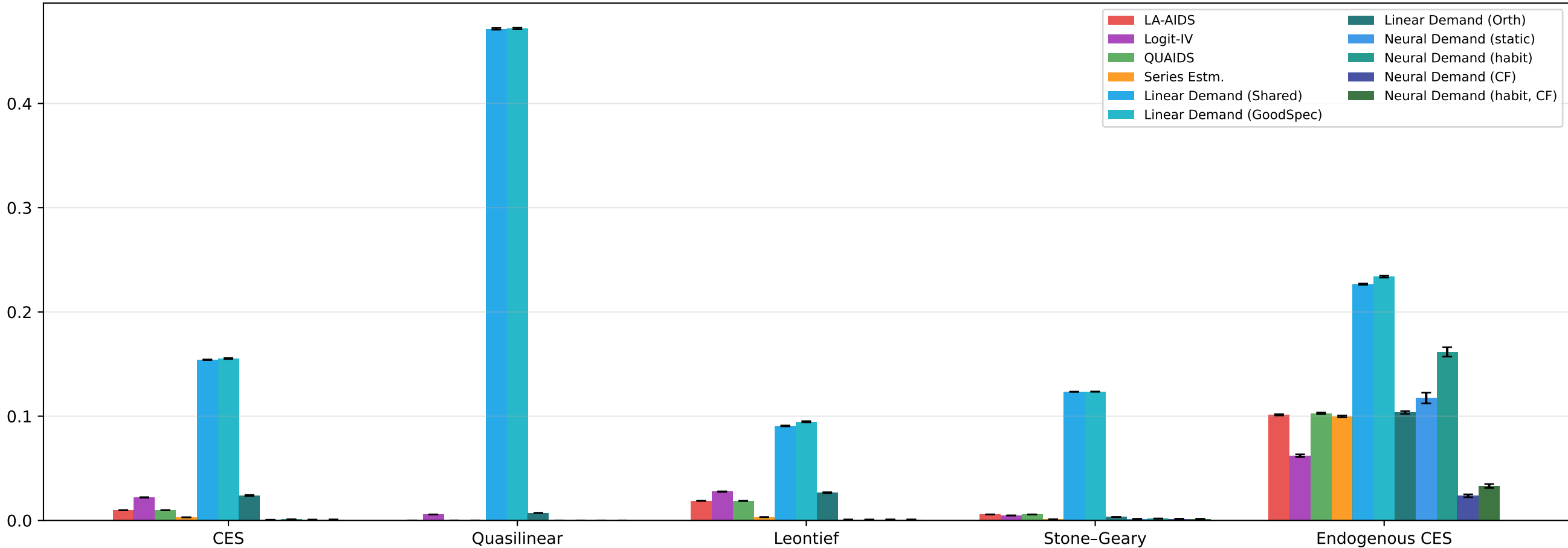
Post-shock RMSE
