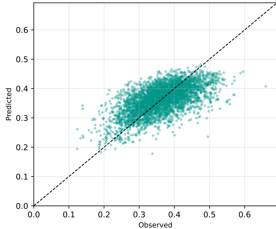
Ibuprofen RMSE=0.0522
