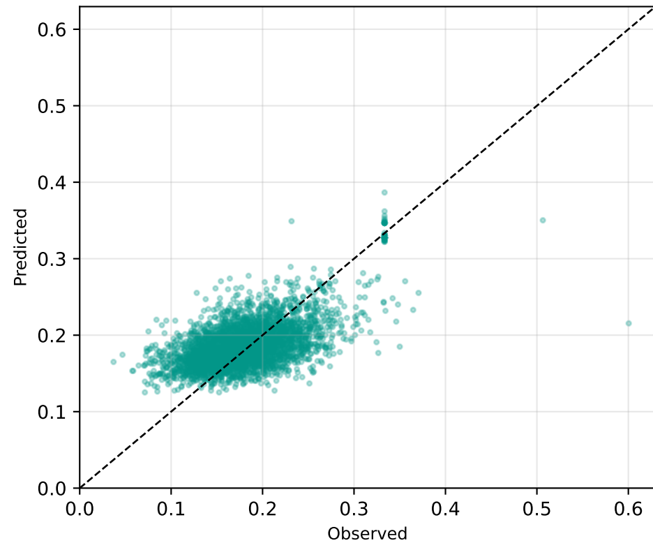
Aspirin RMSE=0.0368
