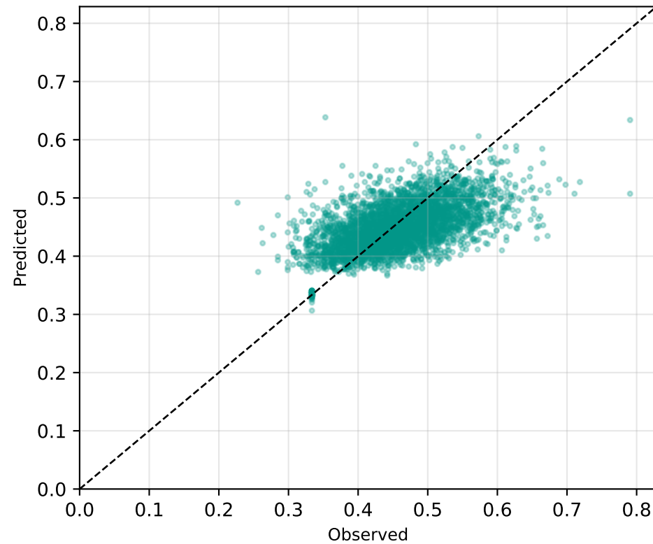
Acetaminophen RMSE=0.0534
