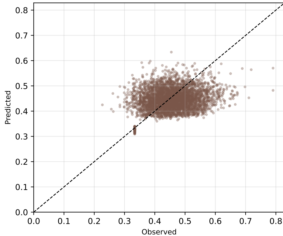
Acetaminophen RMSE=0.0701
