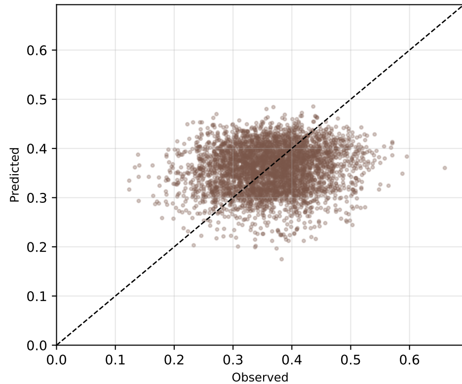
Ibuprofen RMSE=0.0759
