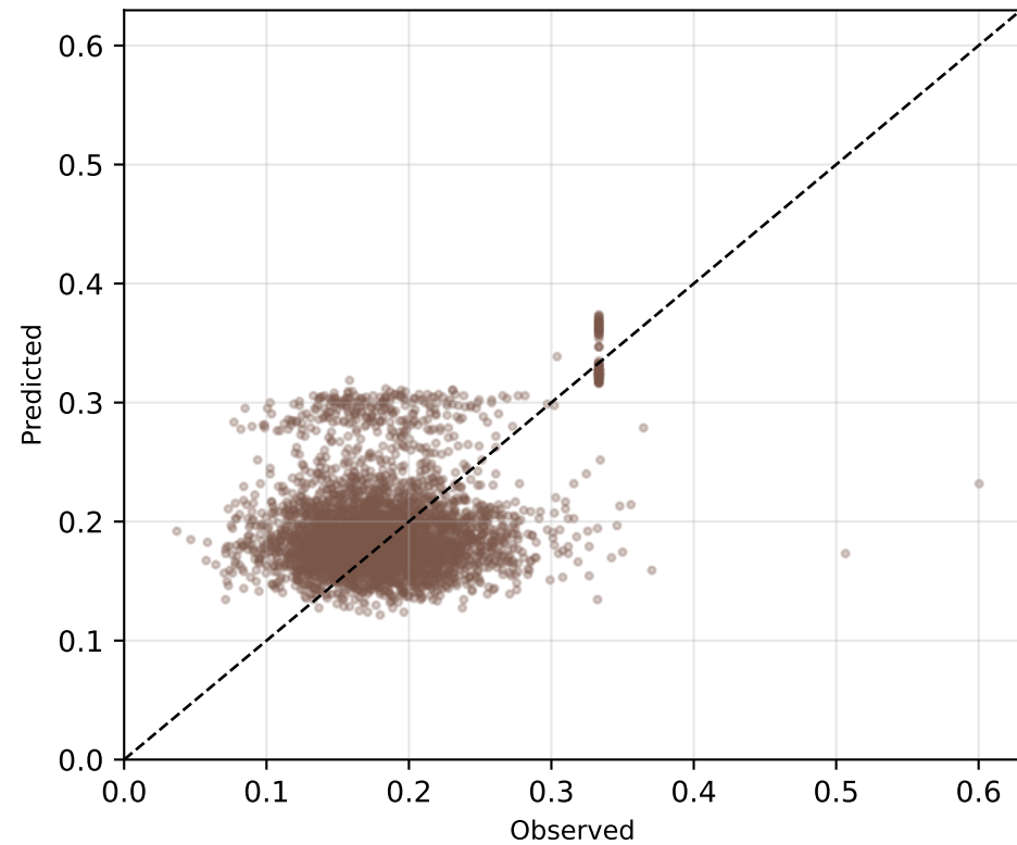
Aspirin RMSE=0.0544
