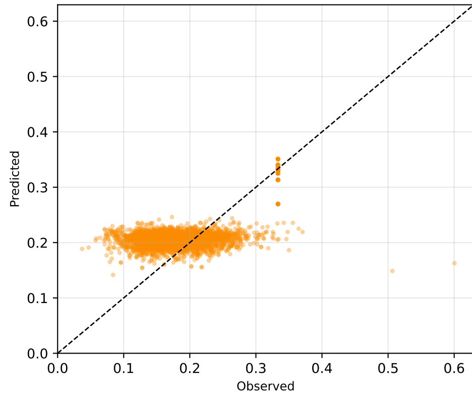
Aspirin RMSE=0.0499
