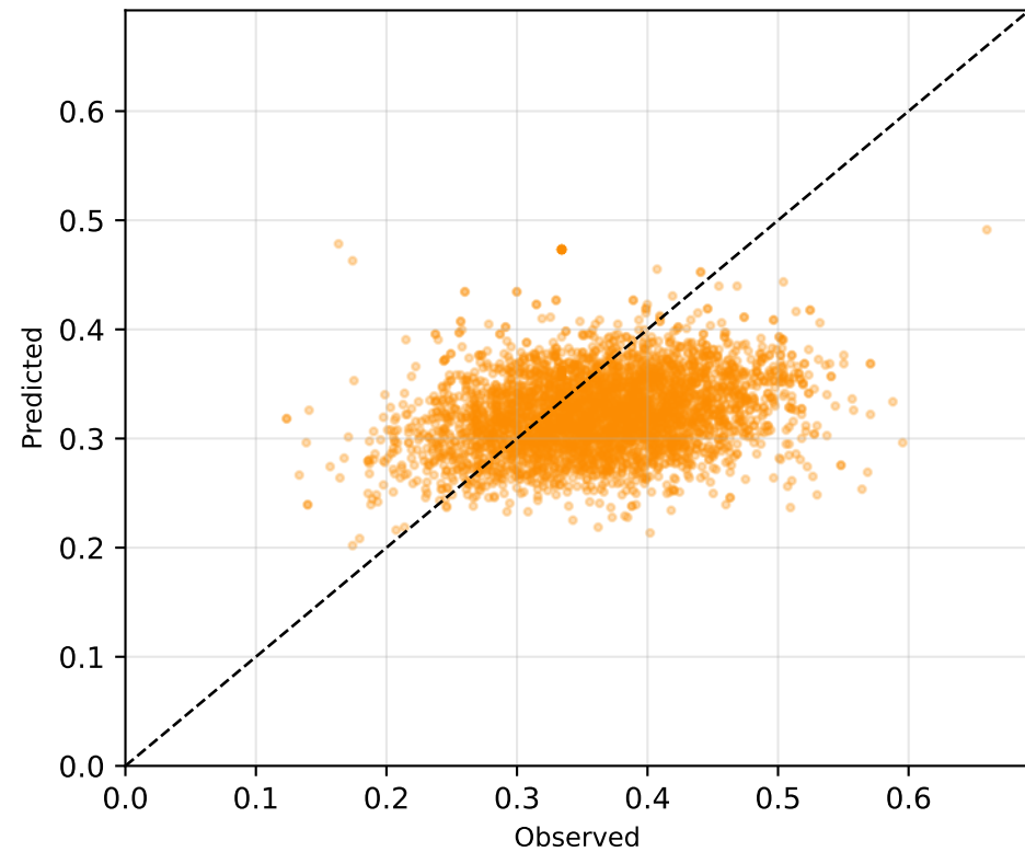
Ibuprofen RMSE=0.0780
