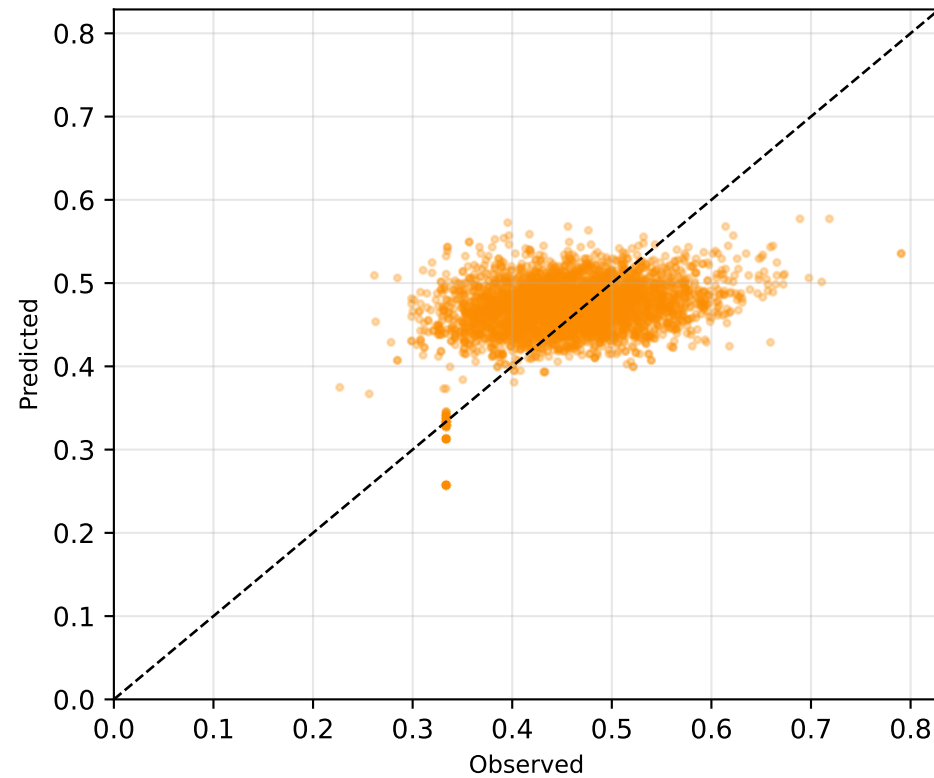
Acetaminophen RMSE=0.0644
