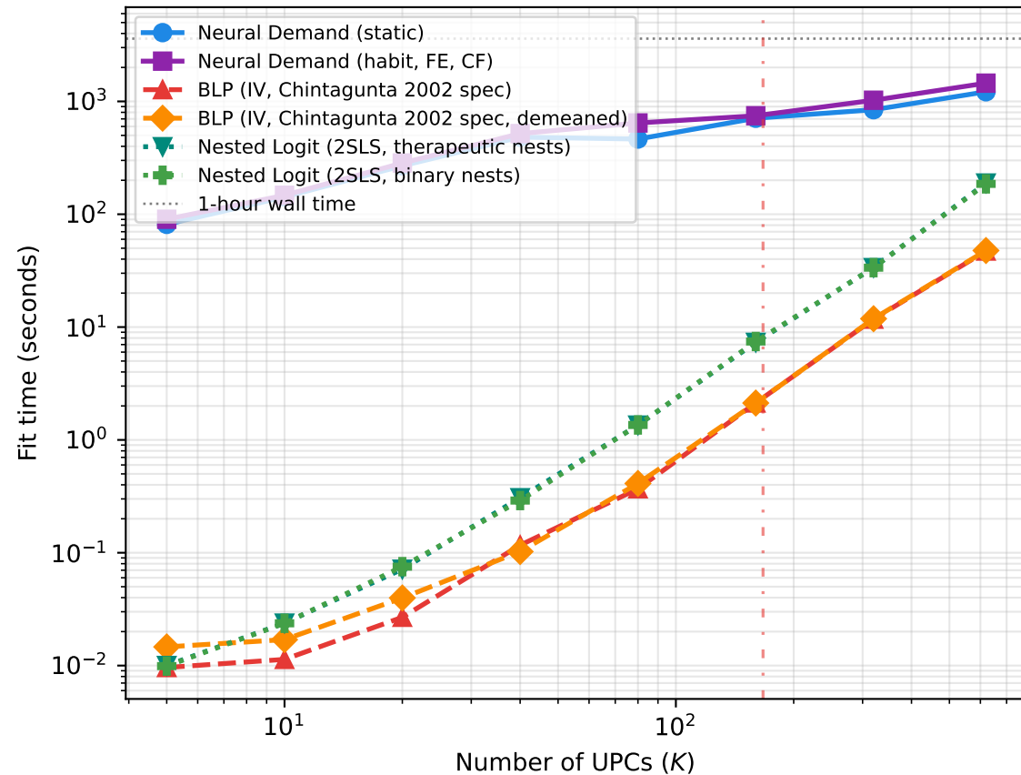
Fit Time vs K (log-log)
