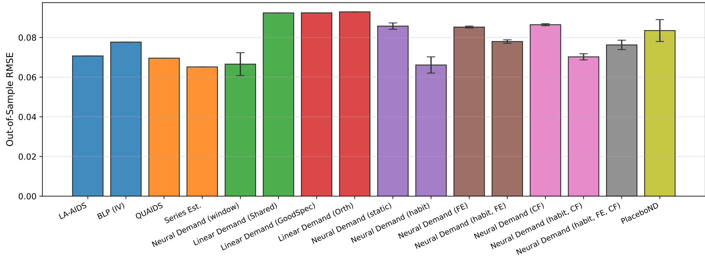
Out-of-Sample RMSE — Mean \pm 1 SD (2 runs) Dominick's Analgesics
