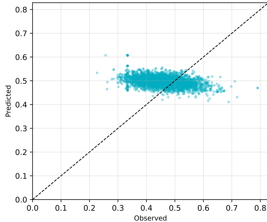
Acetaminophen RMSE=0.0947
