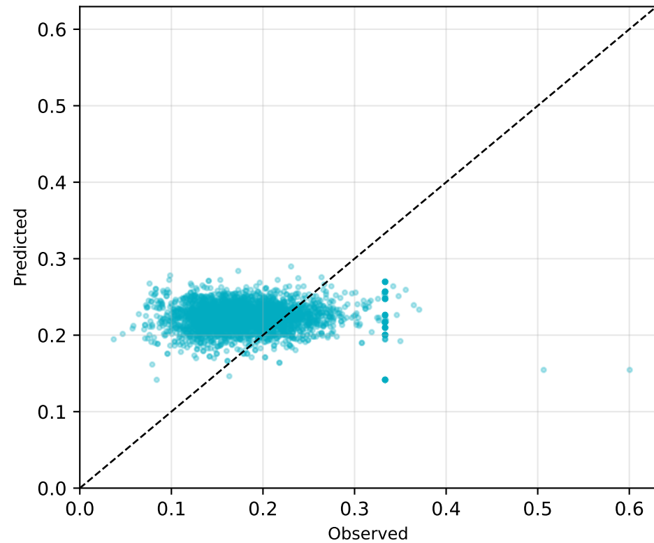
Aspirin RMSE=0.0690
