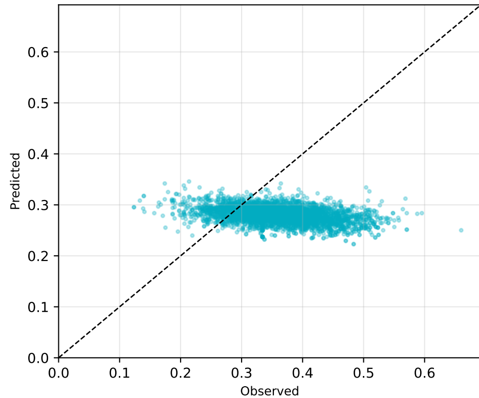
Ibuprofen RMSE=0.1103
