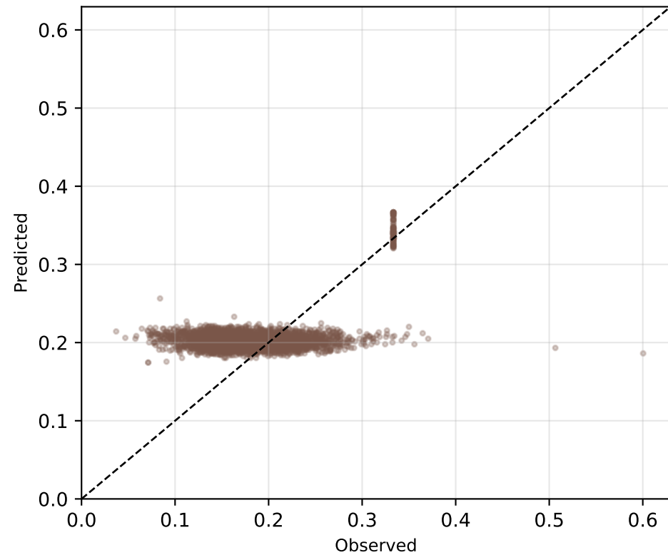
Aspirin RMSE=0.0481
