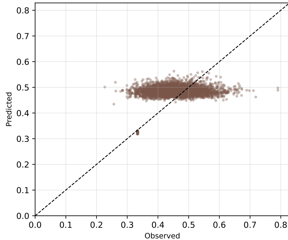
Acetaminophen RMSE=0.0693
