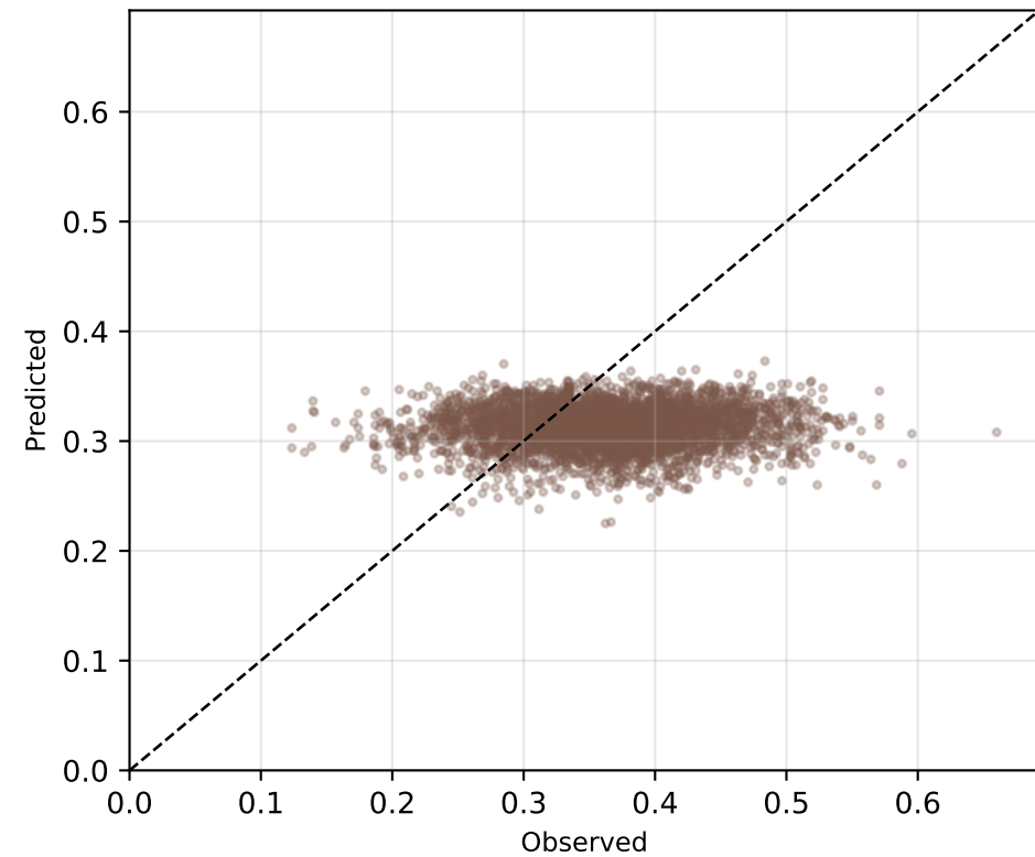
Ibuprofen RMSE=0.0837
