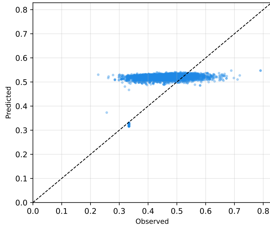
Acetaminophen RMSE=0.0863
