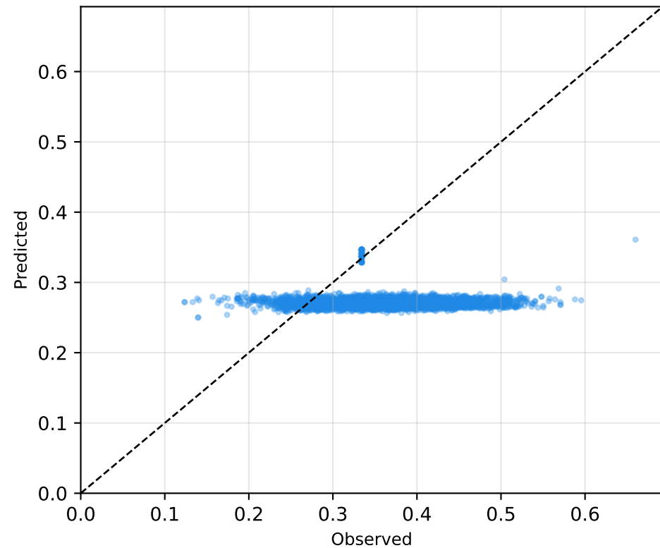
Ibuprofen RMSE=0.1119
