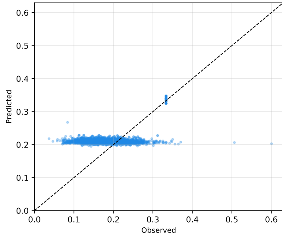
Aspirin RMSE=0.0516
