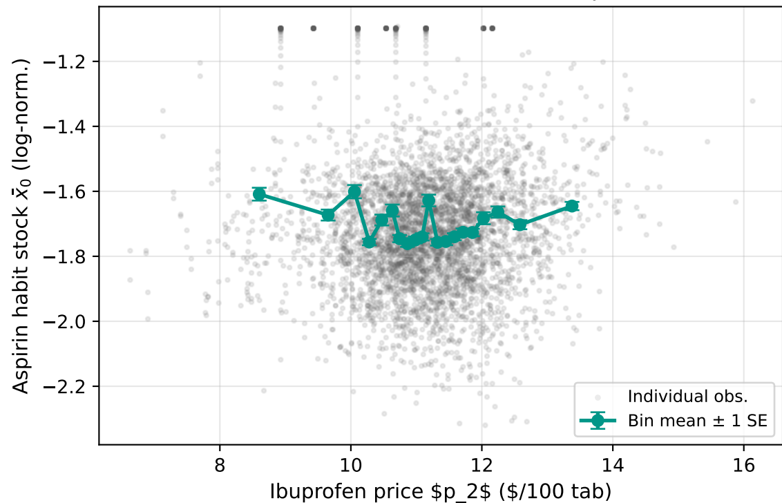
Habit sorting: high-Ibuprofen-price stores have lower aspirin habit Test set (first-in-store obs. excluded) | \rho = -0.033
