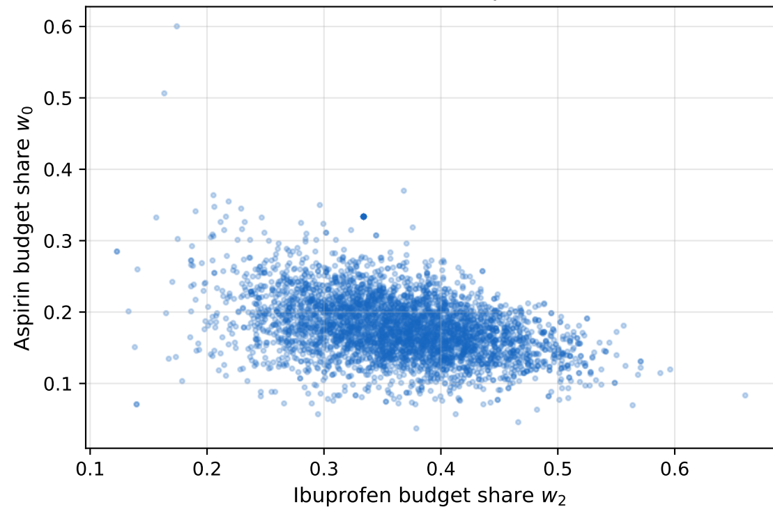
Market segmentation: Aspirin vs Ibuprofen Test-set store \times weeks | \rho = -0.361
