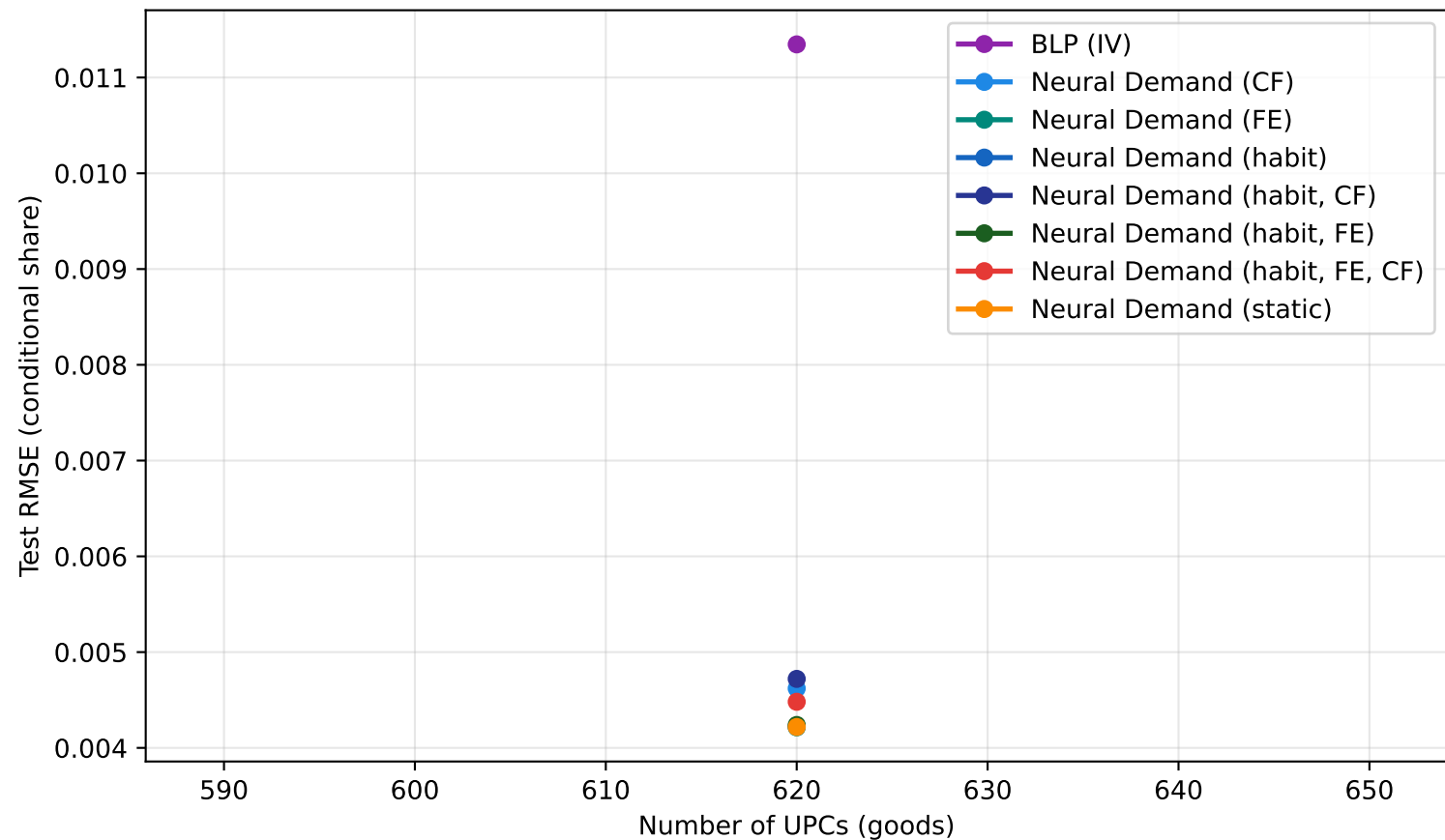
Test RMSE vs Number of Goods
