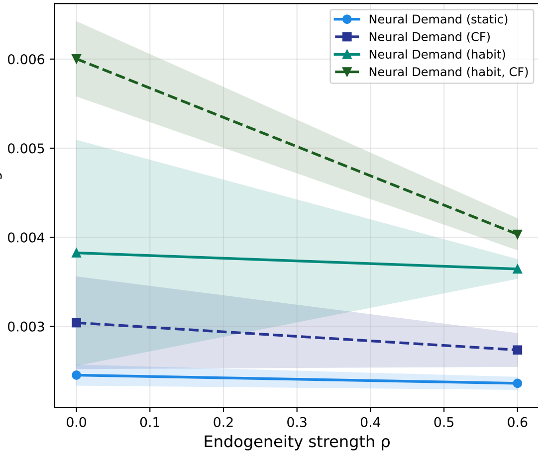
RMSE vs structural ground truth
