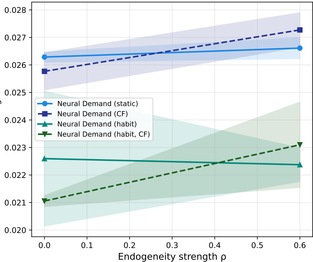
RMSE vs structural ground truth
