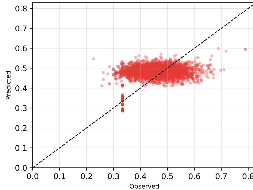
Neural IRL — Acetaminophen RMSE = 0.0644
