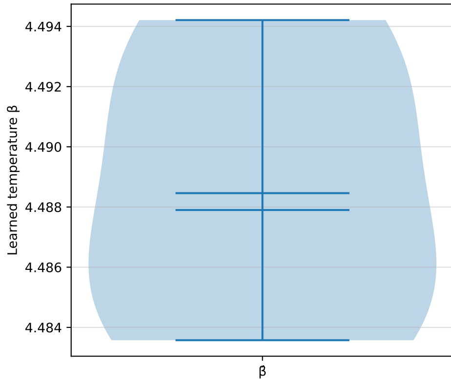
Neural IRL — \beta across runs mean= 4.488 \pm 0.005
