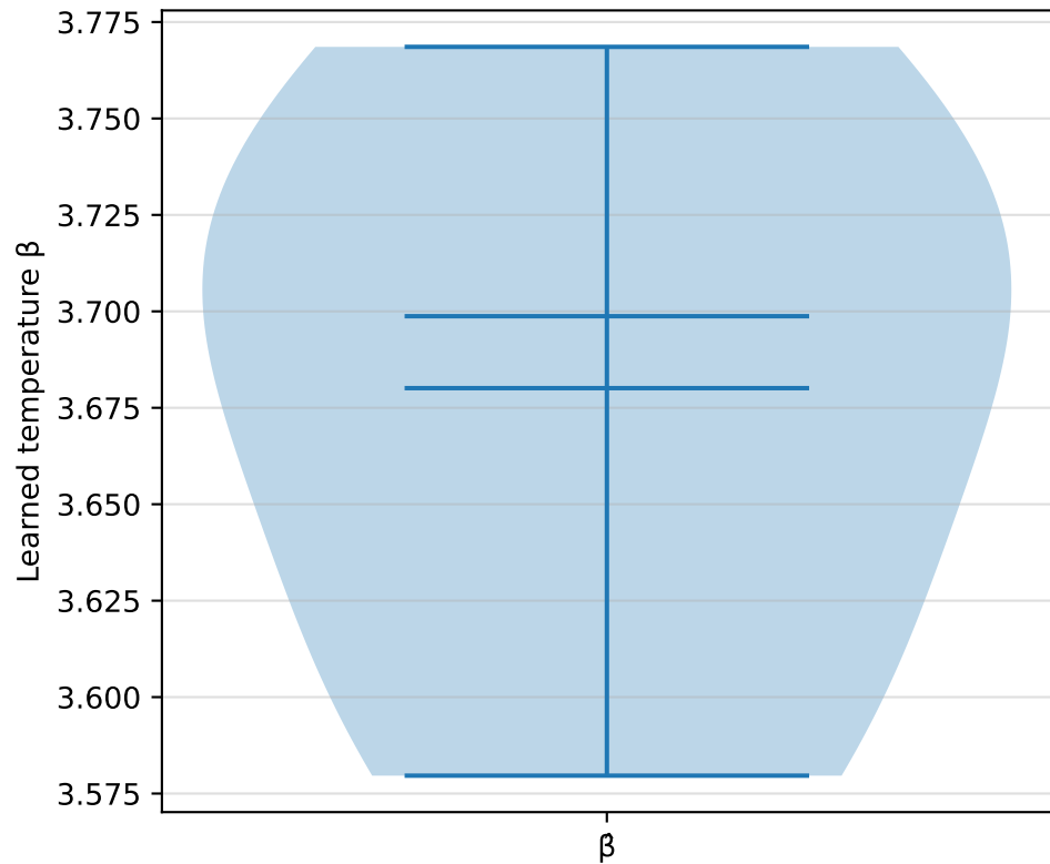
Neural IRL — \beta across runs mean=3.680 \pm 0.074
