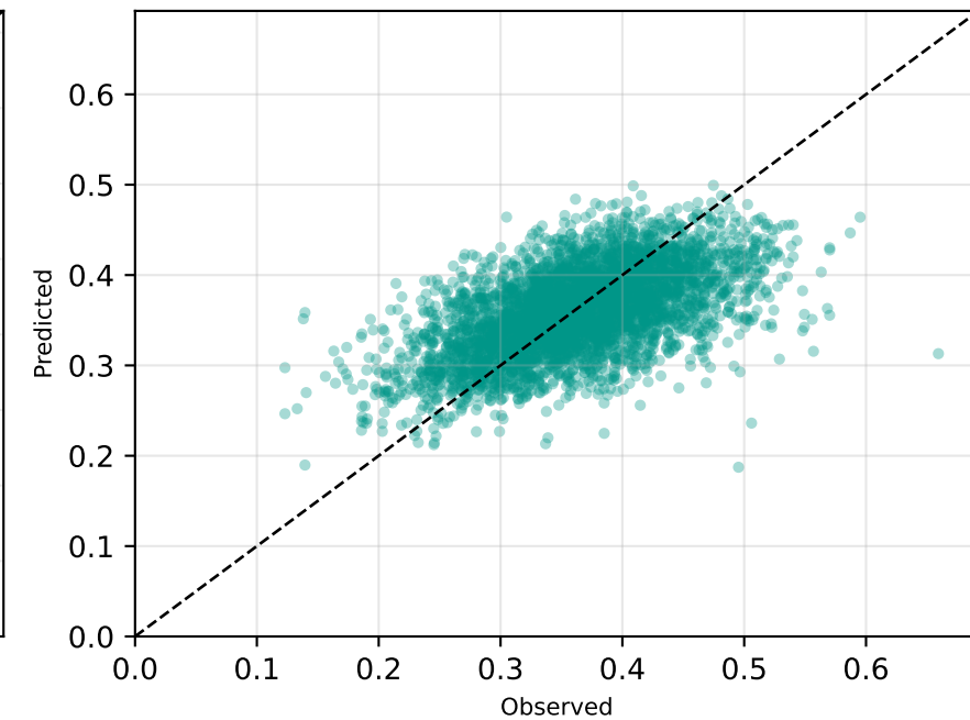
MDP Neural IRL — Ibuprofen RMSE = 0.0556
