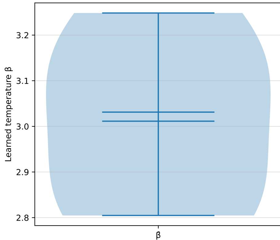
MDP Neural IRL — \beta across runs mean=3.011 \pm 0.190
