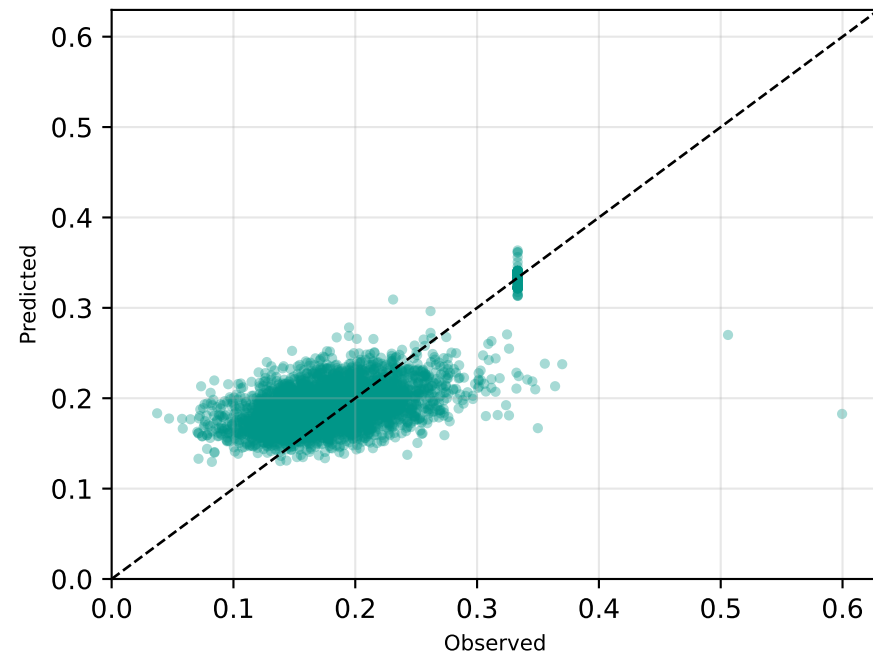
MDP Neural IRL — Aspirin RMSE = 0.0392
