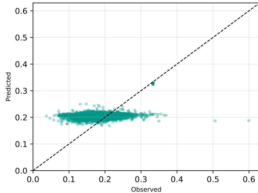
MDP Neural IRL — Aspirin RMSE = 0.0481
