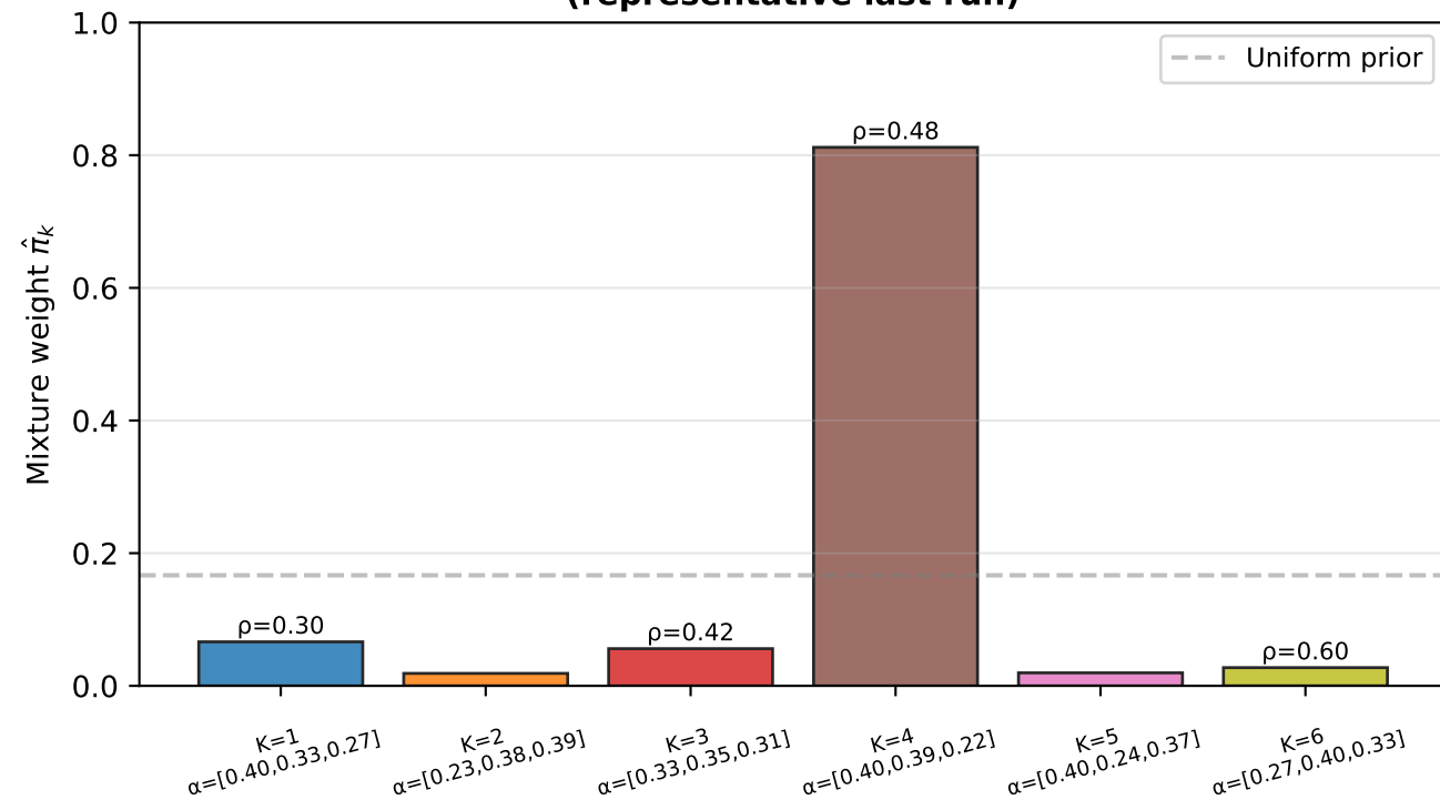
Variational Mixture: Component Weights \hat{\pi}_k (representative last run)
