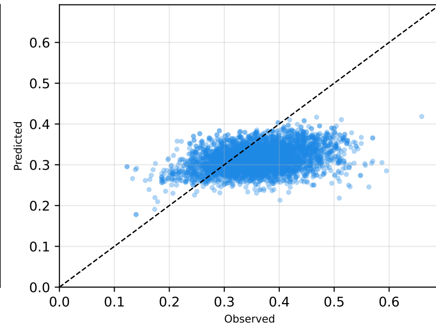
MDP Neural IRL — Ibuprofen RMSE = 0.0709
