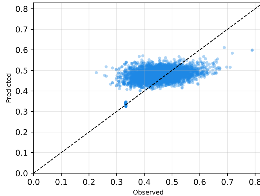
MDP Neural IRL — Acetaminophen RMSE = 0.0562
