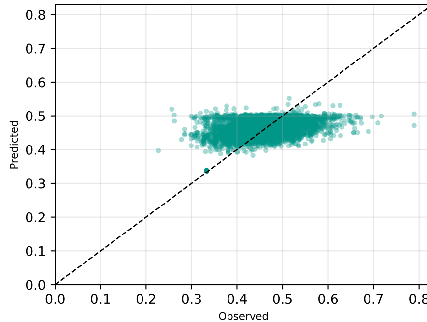
MDP Neural IRL — Acetaminophen RMSE = 0.0605
