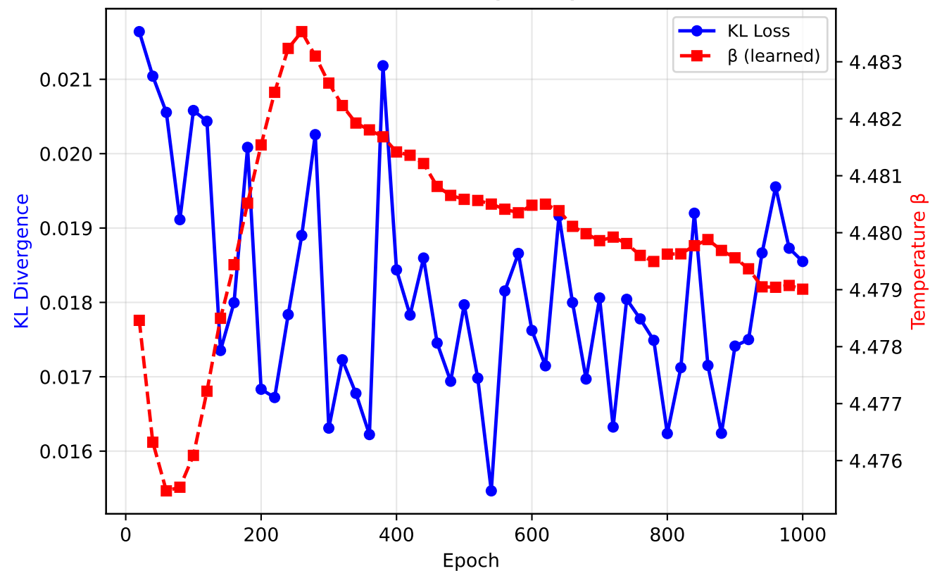
Neural IRL (Static)
