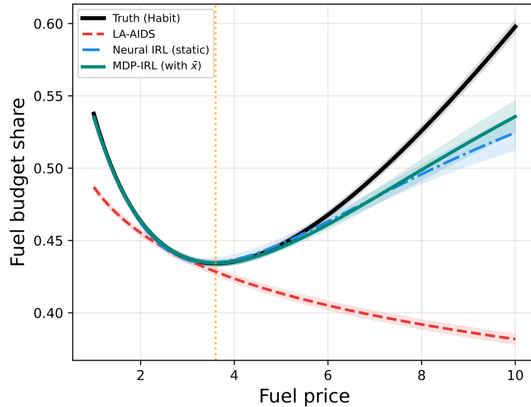
MDP-Aware Neural IRL vs Static Models — Habit Formation DGP Mean \pm 1 SE over 5 runs
