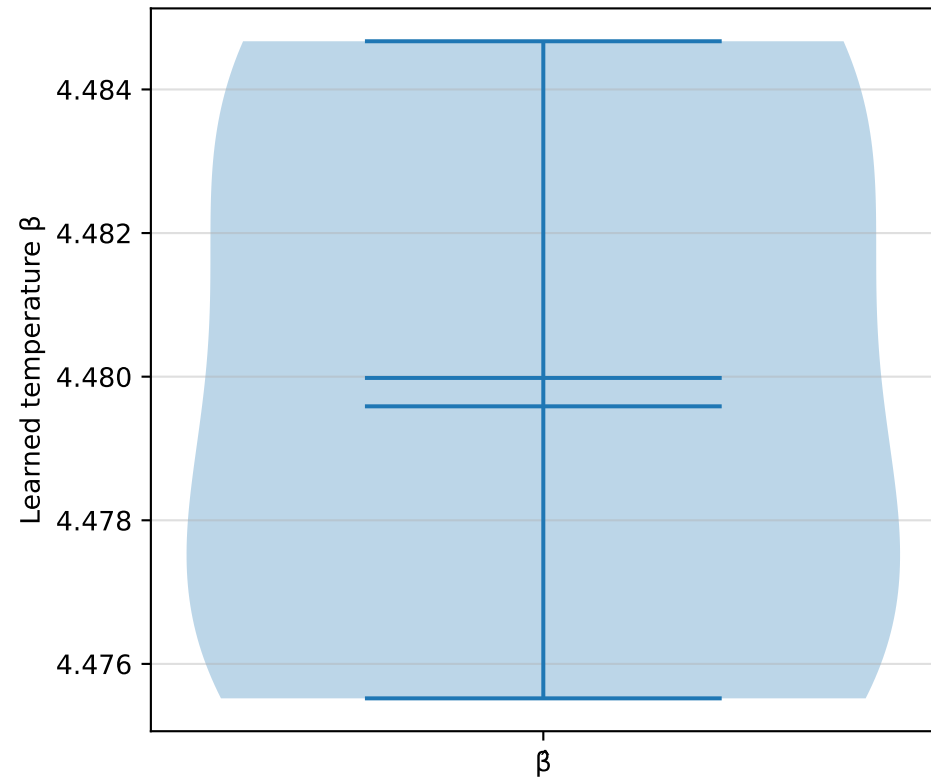
Neural IRL — \beta across runs mean= 4.480 \pm 0.004
