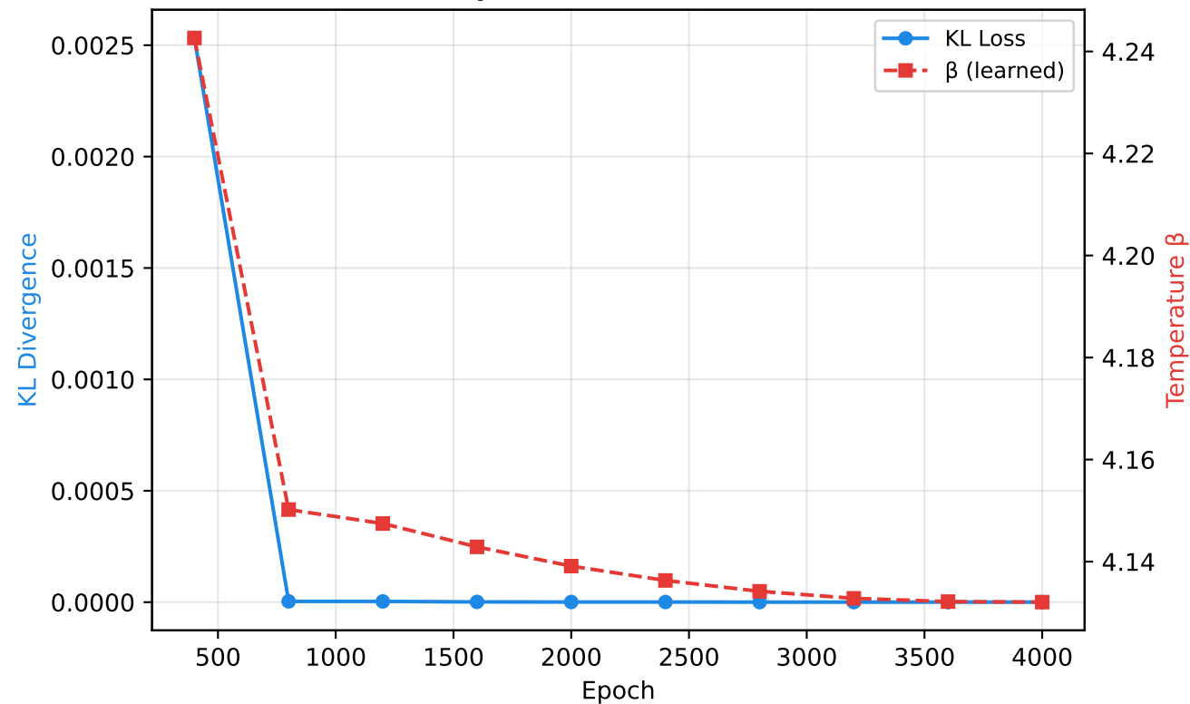
Neural IRL (CES DGP) (representative last run)
