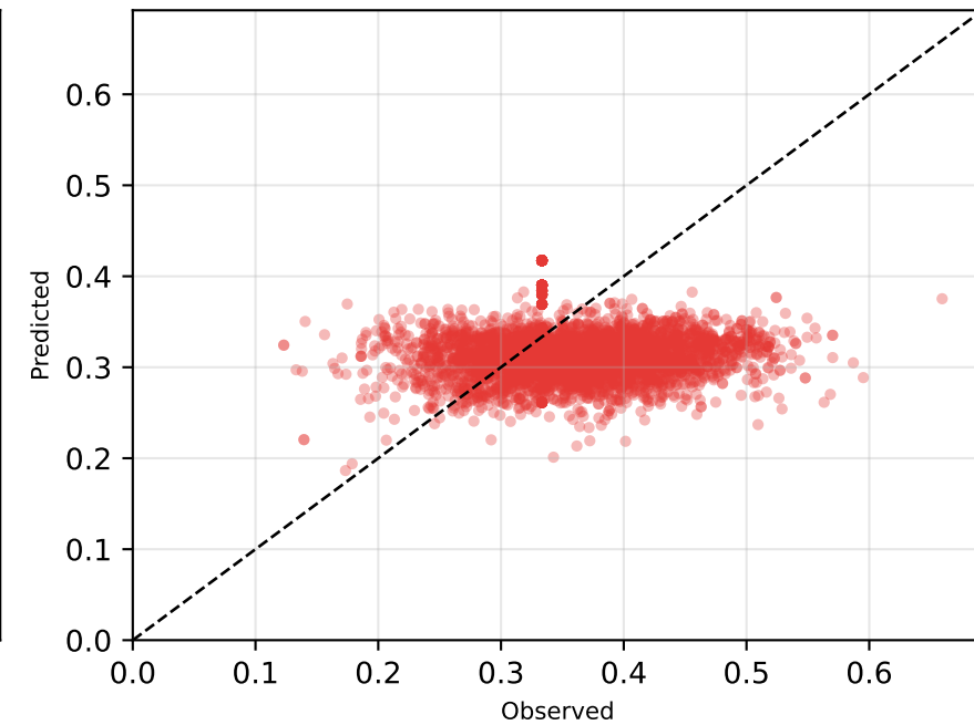
Neural IRL — Ibuprofen RMSE = 0.0784
