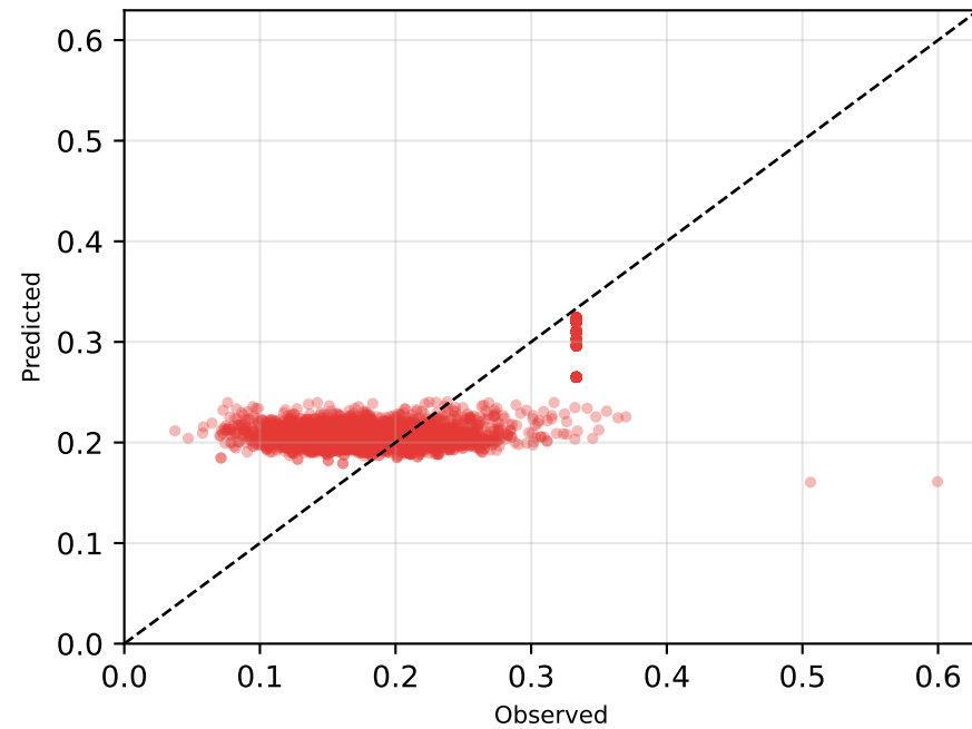
Neural IRL — Aspirin RMSE = 0.0494
