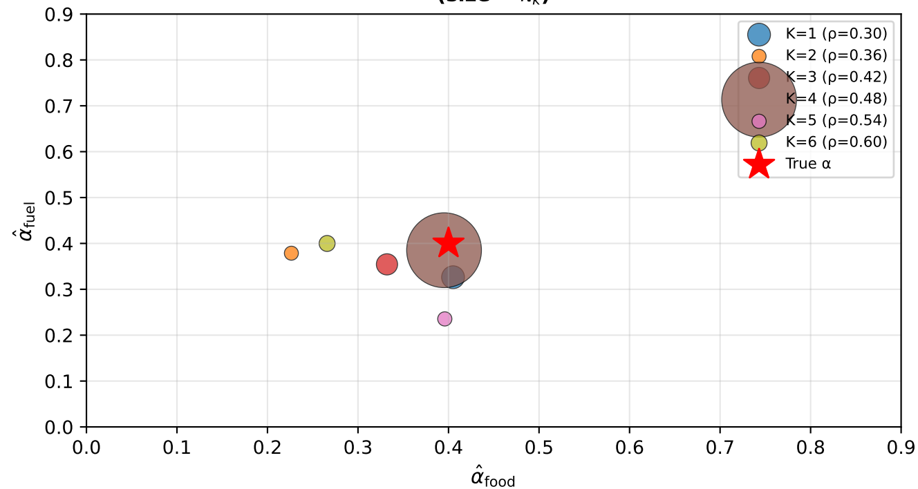
Component Centres in (\hat{\alpha}_{\text{food}}, \hat{\alpha}_{\text{fuel}}) Space (size \propto \hat{\pi}_k )
