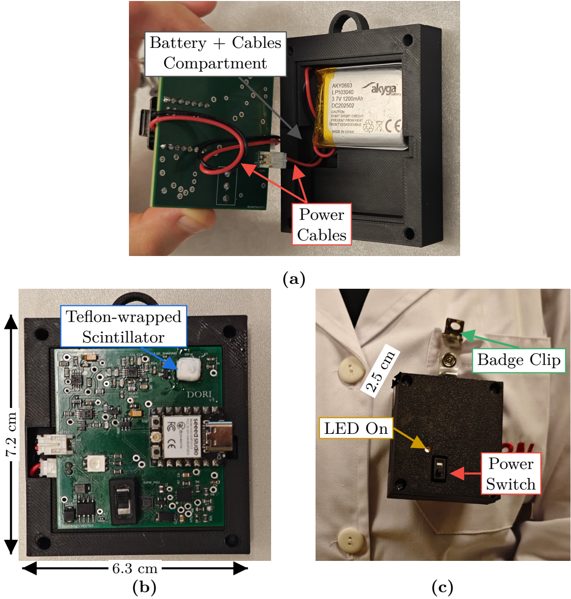
Figure 22: Final DORI prototype. (a) Bottom layer of the enclosure, with the compartment holding the LiPo battery and the cables that connect it to the board. (b) Assembled PCB, with the Tefflon-wrapped scintillator coupled to the SiPM. (c) Closed prototype worn over a lab coat, with the badge clip, the power switch and the LED on.
