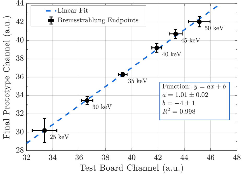
Figure 23: Linear fit of the Bremsstrahlung endpoint channels recorded by the final prototype against those recorded by the DORI-test board, for the tube voltages common to both acquisitions.
