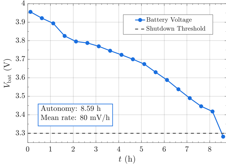
Figure 24: DORI discharge curve during continuous operation at 100 interrupts/second.
