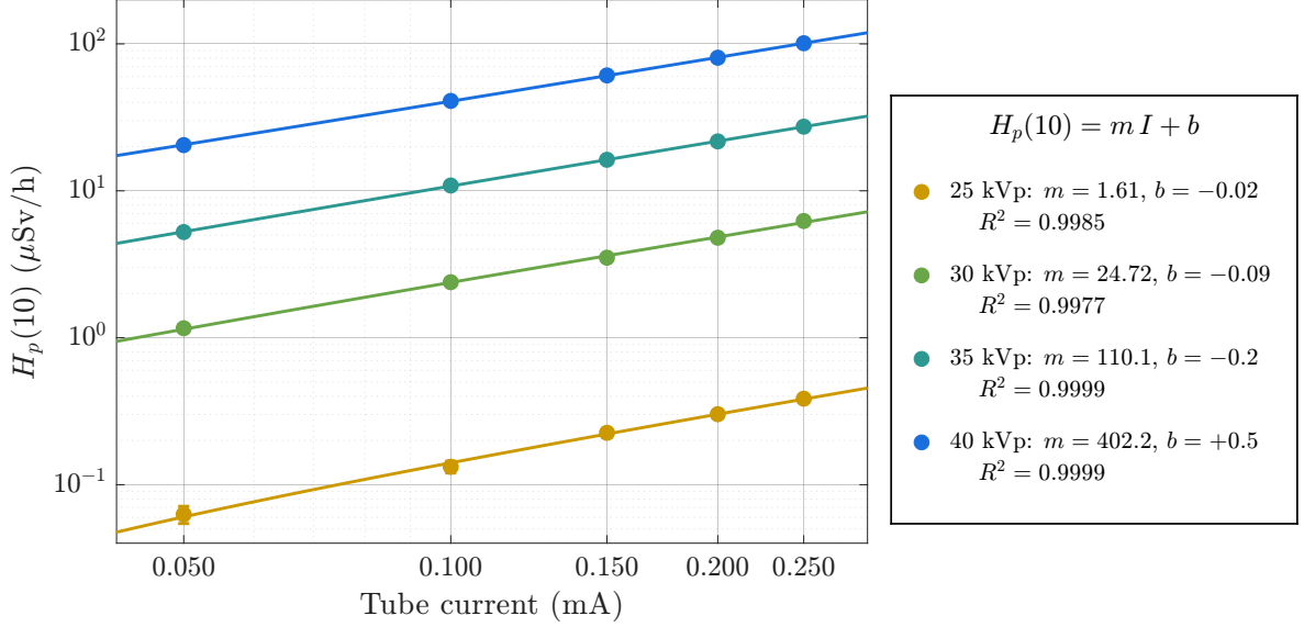
Figure 21: Reconstructed H_p(10) rate as a function of tube current, for tube potentials of 25-40 kVp and currents of 0.050-0.250 mA.
