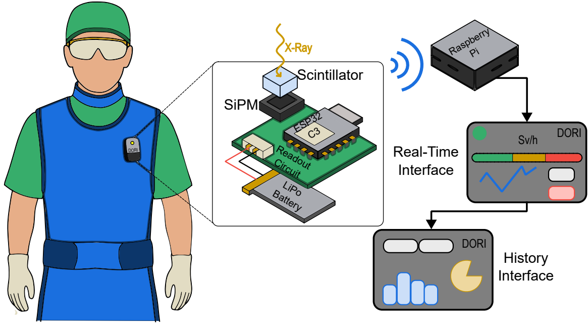
Figure 4: Conceptual design of the DORI system. The wearable unit (exploded view) is worn over the protective apron and comprises the scintillator, photodetector, readout circuit, MCU and LiPo battery. Data are sent to a Raspberry Pi, which displays the real-time and history interfaces.
