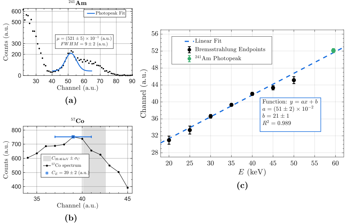
Figure 10: (a) ^{241}\text{Am} spectrum, background subtracted, with the Gaussian fit to the 59.5 keV photopeak. The annotated centroid and FWHM are the mean of five acquisitions, with the maximum deviation from the mean as uncertainty. (b) ^{57}\text{Co} spectrum in the region of the Compton edge of the 122 keV line. The band marks the channel at which the calibration predicts the 39.46 keV edge, within its propagated uncertainty. (c) Weighted least-squares calibration fit to the seven Bremsstrahlung endpoints and the ^{241}\text{Am} photopeak centroid.
