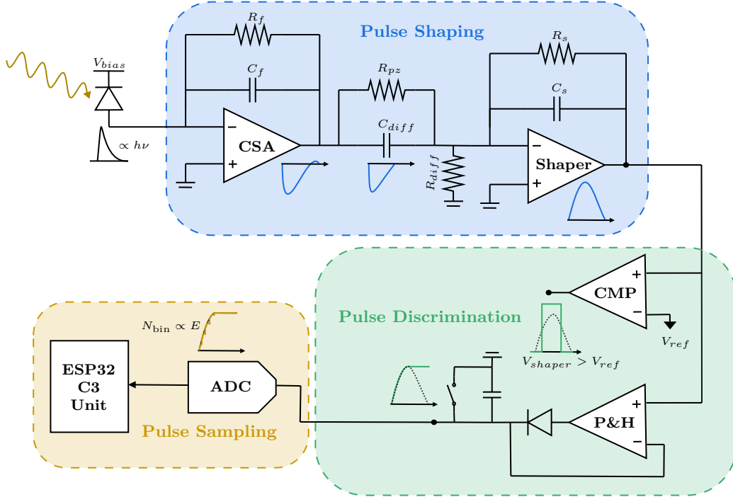
Figure 6: Architecture of the detection system.
