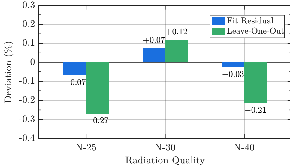
Figure 20: Deviation of the reconstructed \dot{H}_p(10) from the reference value, per radiation quality. Blue bars give the fit residuals, green bars the leave-one-out predictions.
