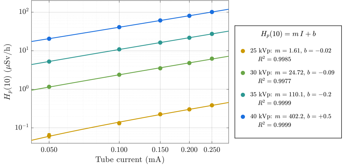
Figure 21: Reconstructed H_p(10) rate as a function of tube current, for tube potentials of 25-40 kVp and currents of 0.050-0.250 mA.
