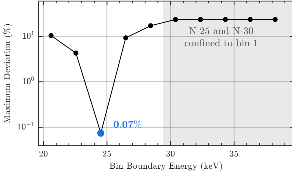
Figure 19: Maximum deviation observed, \delta_{\max} , for each admissible boundary position within the calibrated 20 to 40 keV window.
