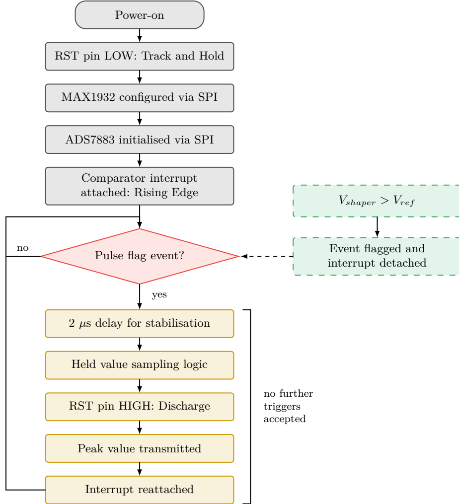
Figure 10: Firmware workflow diagram.
