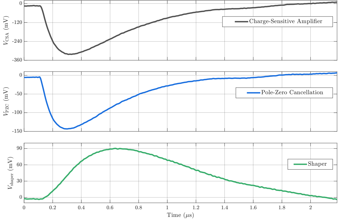
Figure 9: Transient response of the CSA (grey), PZC (blue) and shaper (green) to a single ^{241}\text{Am} event.
