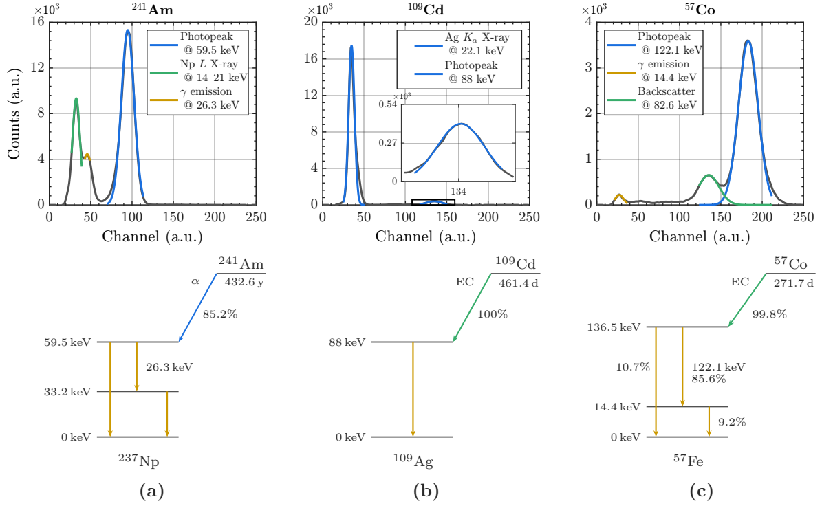
Figure 12: Pulse height spectra acquired with the CsI(Tl) crystal for the three calibration sources, (a) ^{241}\text{Am} , (b) ^{109}\text{Cd} and (c) ^{57}\text{Co} , with the decay scheme of each source beneath.
