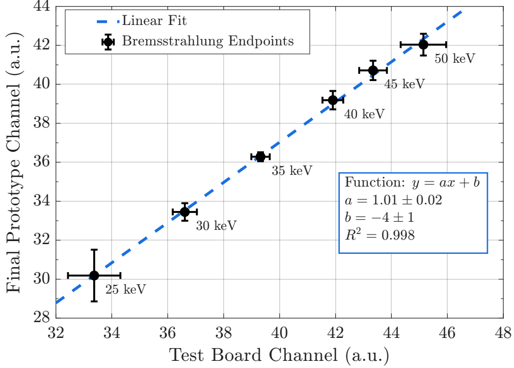
Figure 22: Linear fit of the Bremsstrahlung endpoint channels recorded by the final prototype against those recorded by the DORI-test board, for the tube voltages common to both acquisitions.
