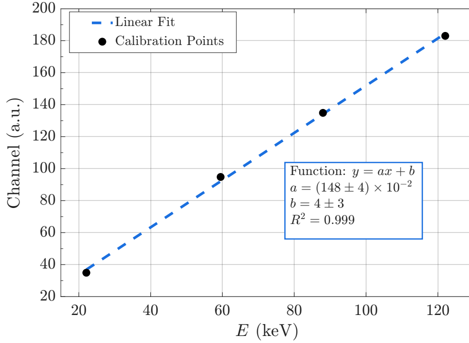
Figure 13: Channel-to-energy calibration of the front-end electronics obtained with the CsI(Tl) crystal, with a linear fit.
