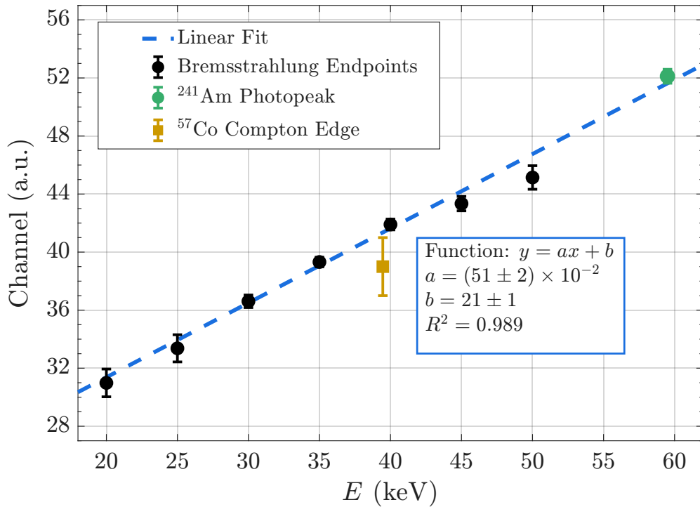
Figure 16: Weighted least-squares energy calibration of the DORI prototype, obtained from the seven Bremsstrahlung endpoints and the ^{241}\text{Am} photopeak centroid. The ^{57}\text{Co} Compton edge is superimposed for validation.
