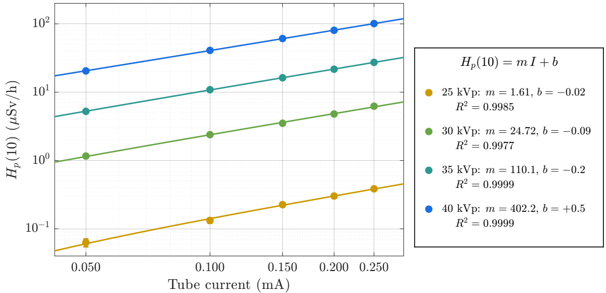
Figure 20: Reconstructed H_p(10) rate as a function of tube current, for tube potentials of 25-40 kVp and currents of 0.050-0.250 mA.
