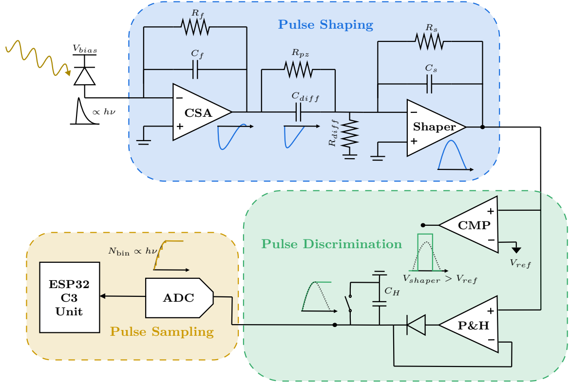
Figure 7: Architecture of the proposed dosimeter.
