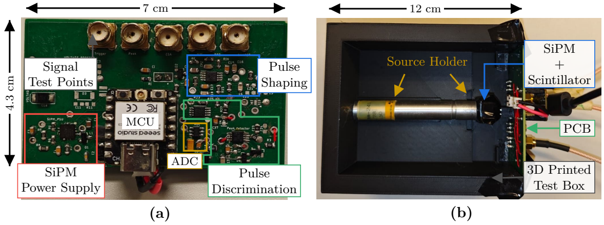
Figure 8: Prototype test board. (a) PCB with the main functional blocks identified, together with the signal test points used for characterisation; (b) assembled prototype inside the 3D-printed test box, showing the sealed source ( ^{241}\text{Am} ) and source holders aligned with the scintillator and SiPM.
