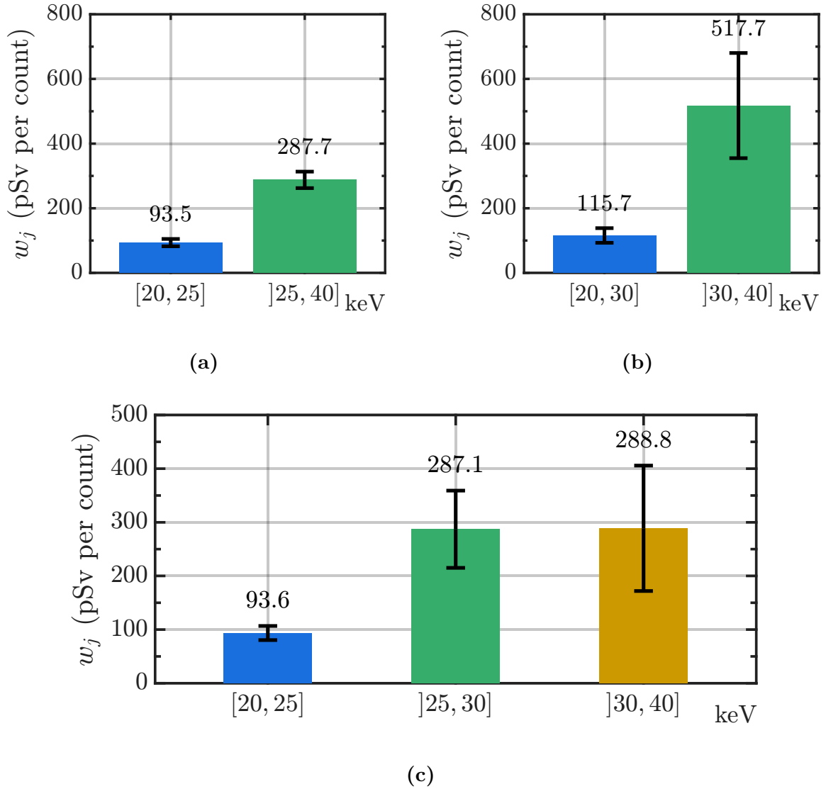
Figure 19: Dose per count obtained for three binning schemes within the calibrated 20 to 40 keV range. (a) Two bins divided at 25 keV; (b) two bins divided at 30 keV; (c) three bins divided at 25 and 30 keV.
