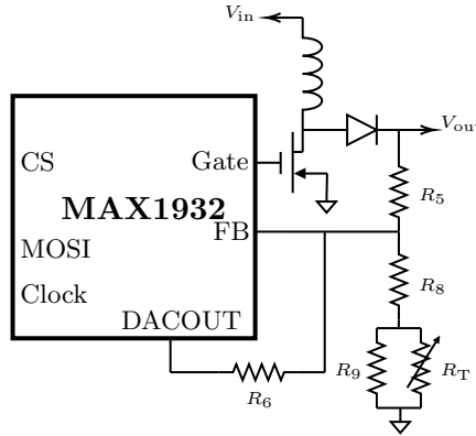
Figure 4: MAX1932 feedback network with the NTC thermistor R_T for temperature compensation of the SiPM bias. Pin labels on the left correspond to SPI connections.
