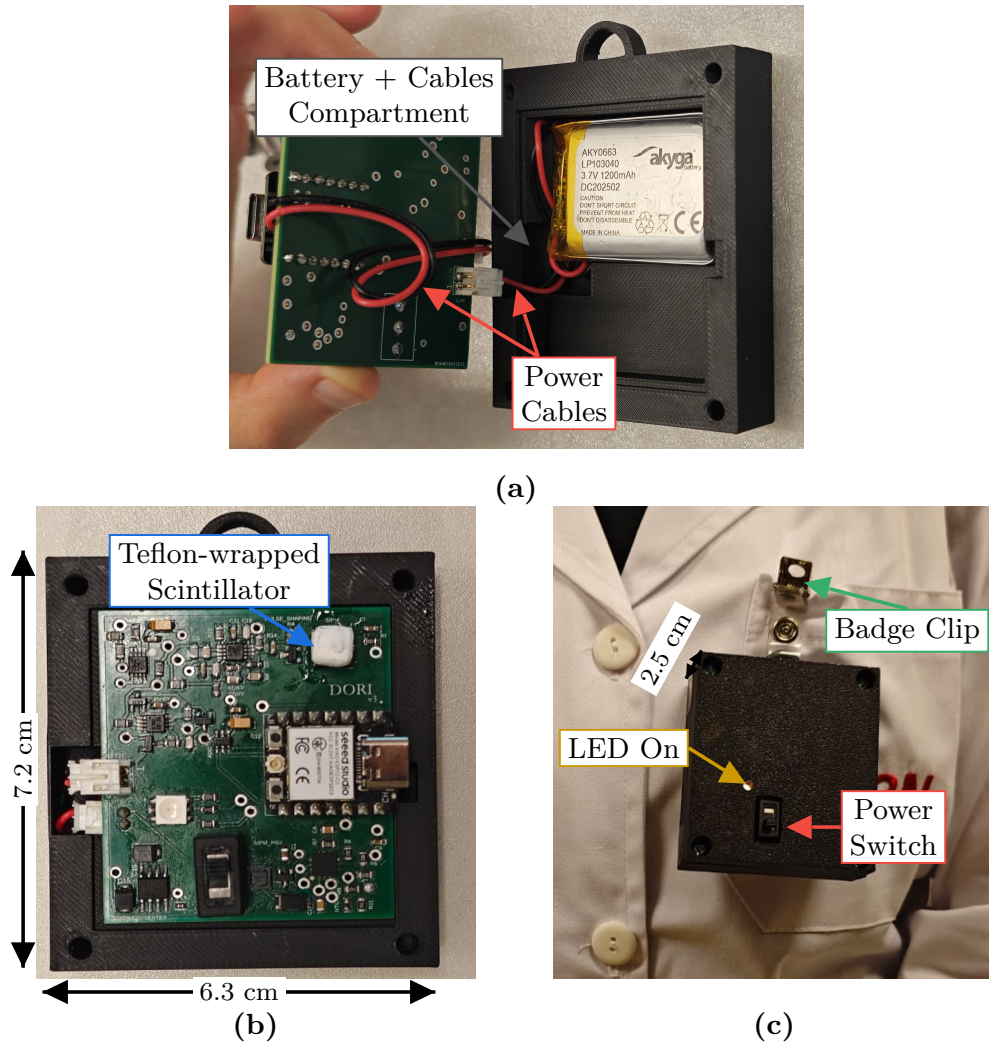
Figure 17: Final DORI prototype.
