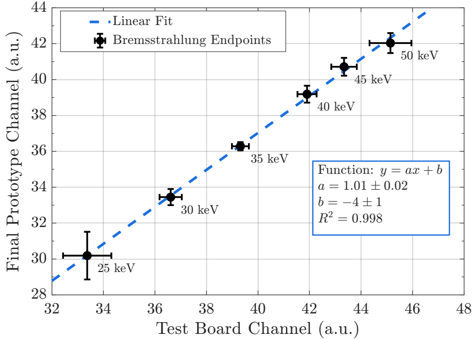
Figure 18: Least-squares fit channel response of the DORI prototype
