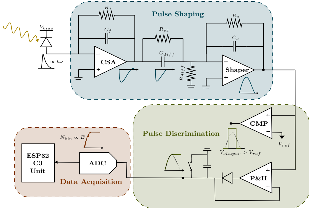
Figure 5: Architecture of the detection system.
