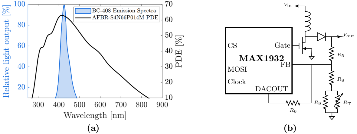
Figure 4: (a) caption (b) MAX1932 feedback network with the NTC thermistor R_T for temperature compensation of the SiPM bias.
