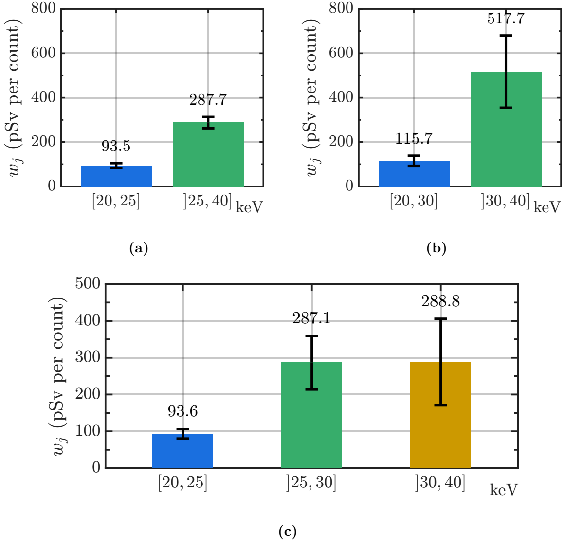
Figure 20: Dose per count obtained for three binning schemes within the calibrated 20 to 40 keV range. (a) Two bins divided at 25 keV; (b) two bins divided at 30 keV; (c) three bins divided at 25 and 30 keV.
