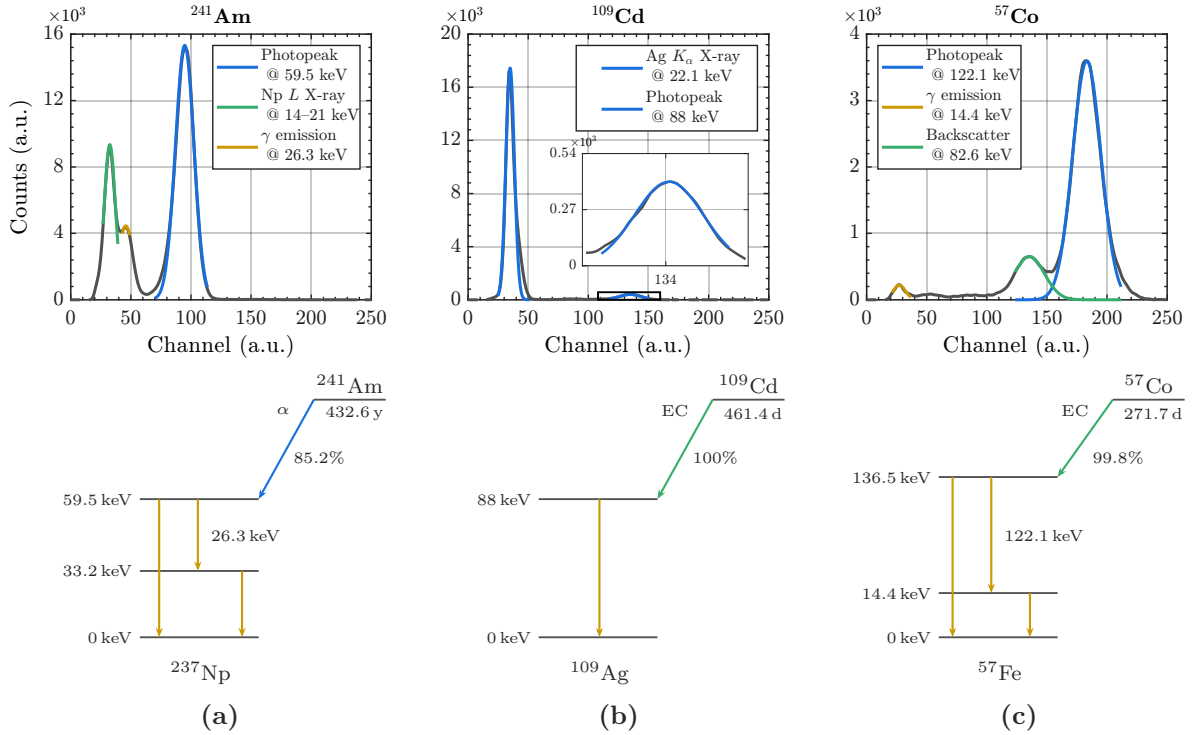
Figure 13: Pulse height spectra acquired with the CsI(Tl) crystal for the three calibration sources, (a) ^{241}\text{Am} , (b) ^{109}\text{Cd} and (c) ^{57}\text{Co} , with the decay scheme of each source beneath. Blue arrows denote \alpha decay, green electron capture and yellow \gamma emission.
