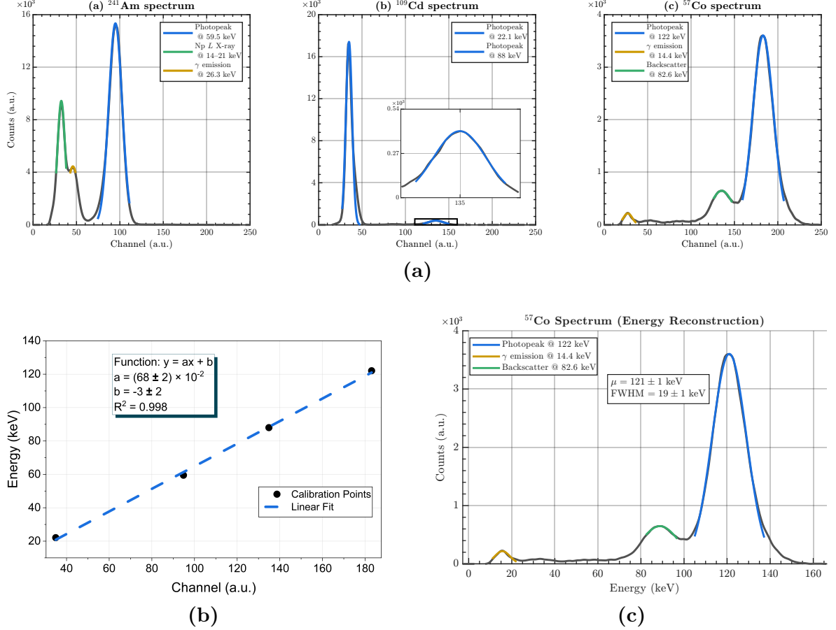
Figure 6: (a) Pulse height spectra acquired with the CsI(Tl) crystal for the three calibration sources. Identified spectral features are labelled. (b) Channel-to-energy calibration curve with linear fit. (c) ^{57}\text{Co} spectrum reconstructed in energy units.
