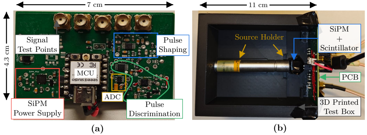
Figure 8: DORI prototype hardware; (a) printed circuit board with the main functional blocks identified, together with the signal test points used for characterisation; (b) assembled prototype inside the 3D printed test box, showing the sealed source holder aligned with the scintillator and SiPM.
