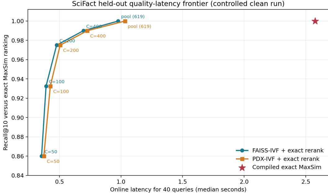
Figure 1: SciFact held-out quality-latency frontier from the controlled clean run (5,183 documents; 40 queries; L = 100 , nprobe = 8 ; four pinned physical cores; median of five interleaved repetitions; online boundary only). Each point is one rerank budget C ; the vertical axis is recall@10 against the exact MaxSim ranking. FAISS-IVF and PDX-IVF trace the same recovery curve, and both reach exact recovery when the full candidate pool ( \approx 619 documents) is reranked, well below the compiled exhaustive latency (star).
