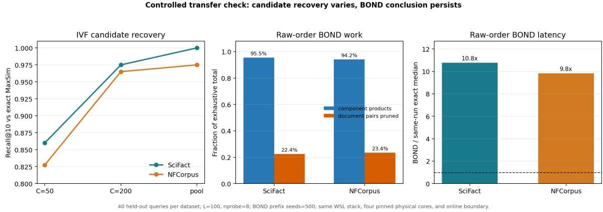
Figure 4: SciFact-to-NFCorpus transfer check (40 held-out queries per dataset; L = 100 , nprobe = 8 ; BOND prefix seeds = 500; same WSL stack, four pinned physical cores, and online boundary). Left: IVF exact-ranking recovery versus rerank budget; NFCorpus saturates at 0.975 because its candidate pool misses part of the exact top-10 for 3 of 40 queries, whereas the SciFact pool is complete. Middle and right: raw-order exact-safe BOND evaluates 94–95% of exhaustive component products and remains about 10 \times slower than the same-run precision-matched exhaustive median on both datasets.
