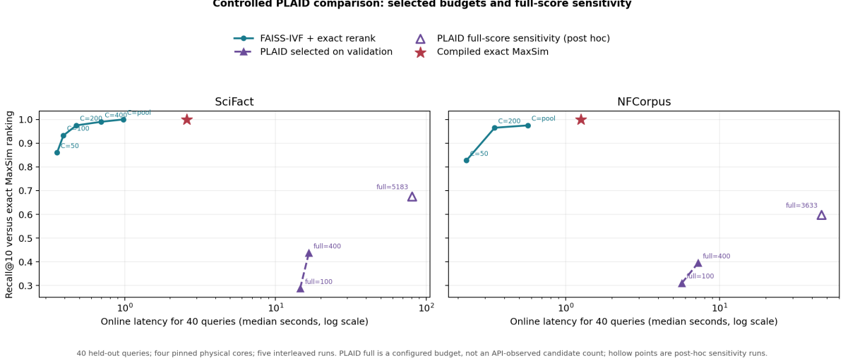
Figure 3: Controlled PLAID results. Selected operating points were frozen on the first 10 SciFact queries before held-out evaluation; the full-corpus score-budget points are explicitly post hoc. Quality is exact recall@10, and latency covers resident normalized query vectors through final ranked document IDs. PLAID is slower and less accurate than compiled exact MaxSim and the IVF frontiers at this tested CPU scale.
