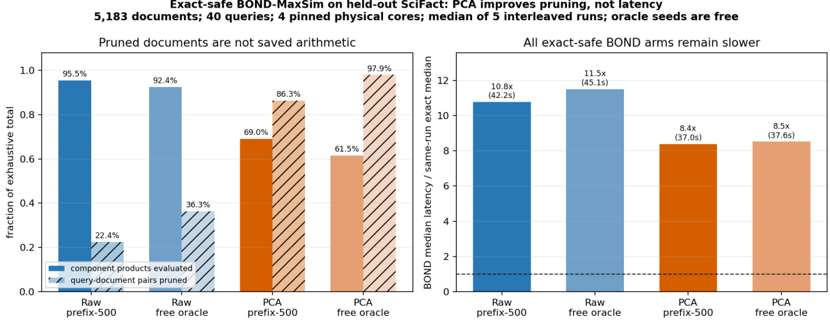
Figure 5: Exact-safe BOND-MaxSim on 40 held-out SciFact queries (5,183 documents; four pinned physical cores; median of five interleaved repetitions; oracle seeds are free and diagnostic). Left: fraction of exhaustive component products evaluated (solid) and query–document pairs pruned (hatched) for raw and PCA-rotated embeddings under prefix-500 and oracle seed policies. Right: BOND median latency relative to the precision-matched exhaustive median of the same run. PCA rotation improves pruning substantially (69.0% and 61.5% of products evaluated) yet every arm remains 8.4–11.5 \times slower than exhaustive scoring.
