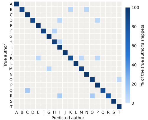
Figure 2: Confusion matrix of the final SVC on the test set, normalized per true author. Authors are labeled A-T.
